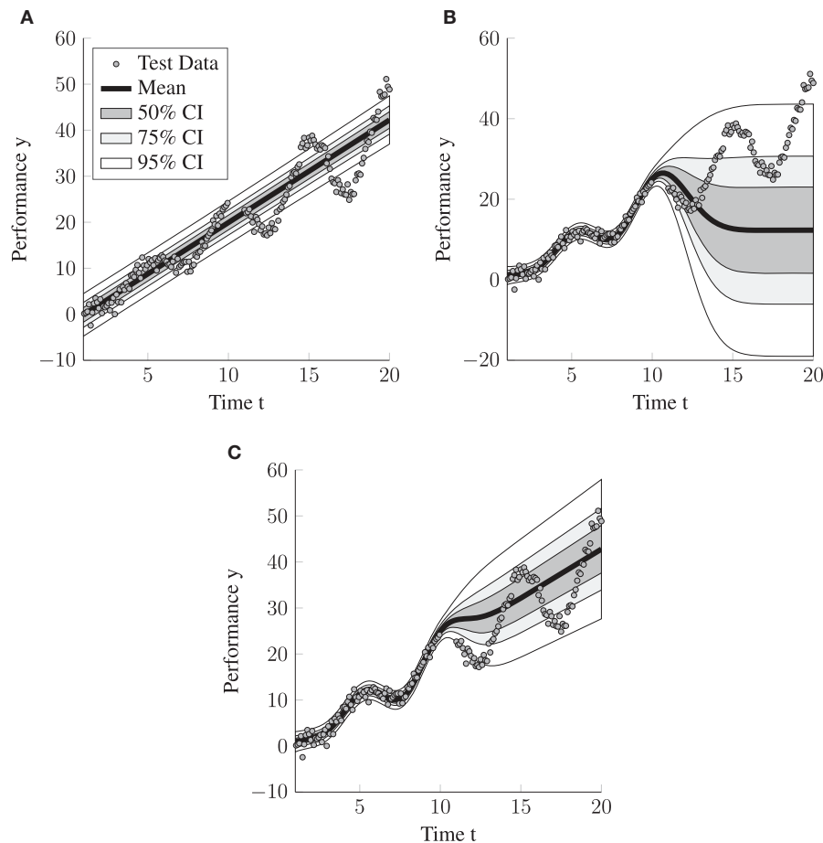
FIGURE 3 | Visualization of the predictive distributions on the data generated from the LGCM + unknown deviation distribution for the three considered models. CI = credibility interval. (A) LGCM. (B) SE Model. (C) LGCM+SE.
