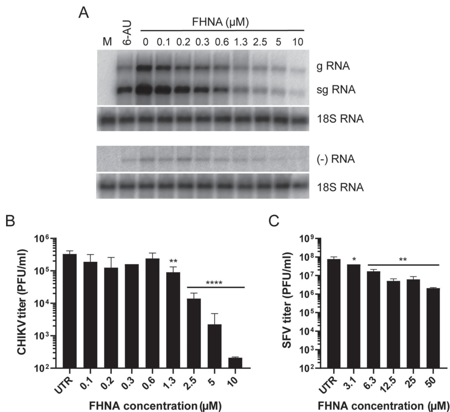
Figure 1. FHNA inhibits CHIKV replication in a dose-dependent manner. (A) VeroE6 cells were infected with CHIKV at an MOI of 1 and treated with 0 to 10 μM FHNA. A 20 μM dose of 6-azauridine was included as a positive control. At 8 hpi intracellular RNA was isolated with TRIzol reagent and subjected to denaturing agarose gel electrophoresis and in-gel hybridization with 32 P-labelled probes specific for positive- and negative-strand CHIKV RNA. 18S rRNA was used as a loading control. (B) VeroE6 cells were pretreated with 0 to 10 μM FHNA for 2 h and then infected with CHIKV at an MOI of 1. After 1 h of incubation, the inoculum was replaced with medium containing 0 to 10 μM FHNA. At 20 hpi, the supernatants were harvested for virus titration by plaque assay. (C) VeroE6 cells were pretreated with 0 to 50 μM FHNA for 2 h and then infected with SFV at an MOI of 5. After 1 h of incubation, the inoculum was replaced with medium containing 0 to 50 μM FHNA. At 8 hpi, the supernatants were harvested for virus titration by plaque assay. UTR, untreated. The data for panels B and C represent the mean ± the standard deviations (SD) of two independent experiments performed in duplicate. Statistical analysis was performed using a one-way ANOVA multiple comparison test. Statistically significant differences are indicated by asterisks (*, P < 0.05 ; **, P < 0.01 ; ***, P < 0.001 ; ****, P < 0.0001 ).
