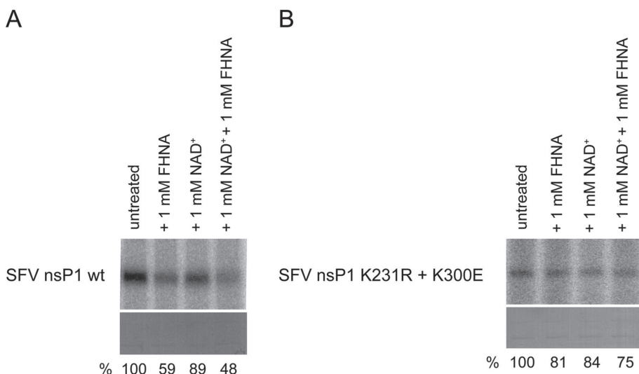
Figure 9. Effect of oxidized FHNA on the activity of wt and mutant SFV nsP1 under nonreducing conditions. (A) wt SFV nsP1 was incubated with [ \alpha^{32}\text{P} ]GTP and 10 \mu\text{M} SAM and was left untreated, incubated with 1 mM FHNA, with 1 mM \text{NAD}^+ , or a combination of 1 mM FHNA and 1 mM \text{NAD}^+ at 30°C for 30 min. The reaction was performed in the absence of DTT and was stopped with 10 % SDS. (B) The reactions as described in panel A were performed with the SFV nsP1 K231R + K300E mutant. In both panels A and B the \alpha^{32}\text{P} -m 7 GMP-nsP1 covalent intermediate was visualized following 7-day exposure of the Phosphorimager screen. The relative activity (expressed as the percentage of untreated control) is indicated below the lanes in panels A and B. It was calculated using QuantityOne software by dividing the volume of the bands of interest by that of the untreated control. Coomassie blue staining was used to demonstrate equal protein loading.
