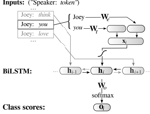
Figure 2: BiLSTM applied to “...think you love...” as spoken by Joey (from Figure 1), outputting class scores for mention “you” (bias b_o not depicted).
