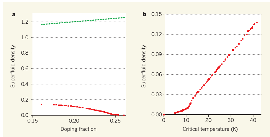
Figure 1 | Surprising superconductivity. Božović et al. 5 have measured key properties of ‘overdoped’ high-temperature copper oxide superconductors. a , From their measurements, the authors estimate the superfluid density (red, corresponding to the number of electrons taking part in superconductivity per unit cell; the unit cell is the smallest periodically repeating structure in a crystal) as a function of the doping fraction (a measure of the density of charge carriers). They observe far fewer superconducting electrons than expected from the Bardeen–Cooper–Schrieffer (BCS) theory (green). b , The data are presented here as a plot of the superfluid density against the critical temperature (the temperature below which the material can superconduct). The superfluid density is directly proportional to the critical temperature, over a wide doping range. The authors’ remarkable results are incompatible with standard BCS theory and require new explanations.
