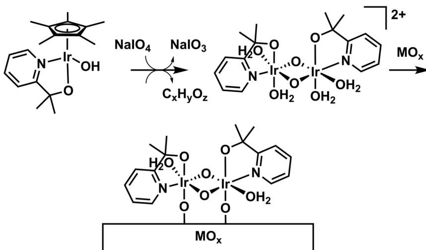
Scheme 1.3. Oxidative degradation and subsequent immobilization of the active species formed by [Cp*Ir(pyale)(OH)]. 102
