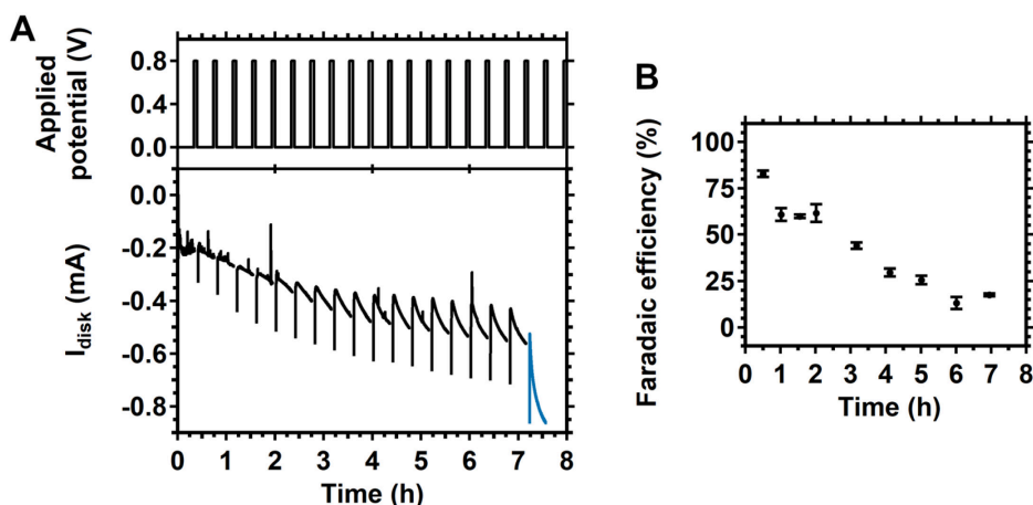
Figure C.11. Rotating disk measurement at 0.0 V of O_2 reduction by Cu_2(btmpa) (A) and the corresponding Faradaic efficiency (B). The full 8 hours of the measurement of Figure 4.6 is depicted. Before the last 20 minutes (blue line in A), the H_2O_2 concentration was manually increased 5 times.
