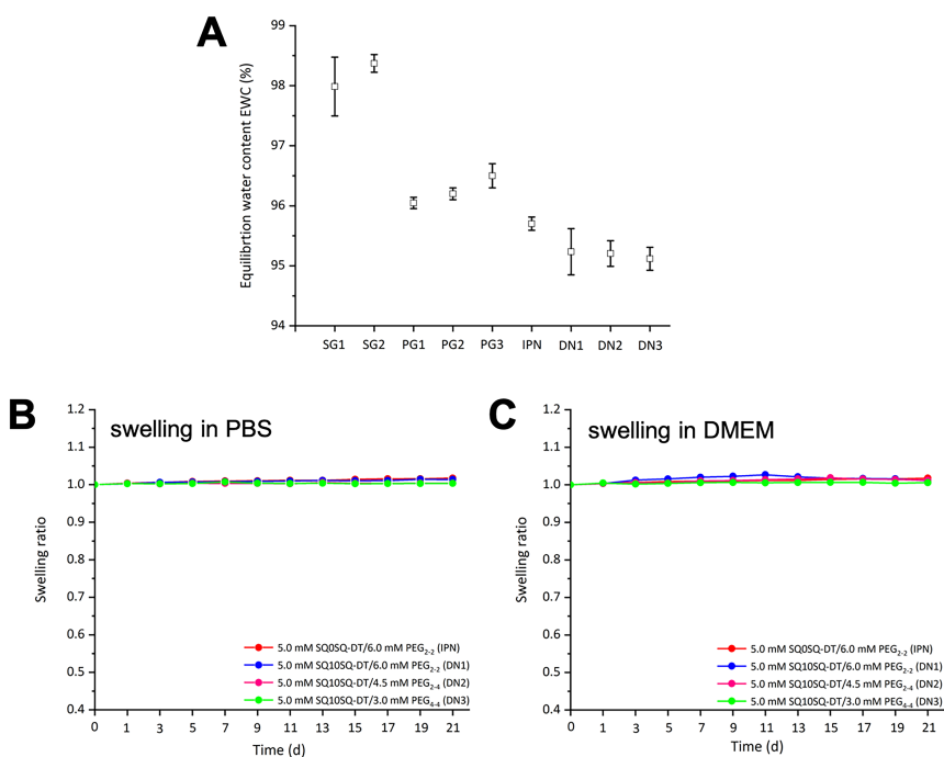
Figure 5.4 (A) Average (N = 3) equilibrium water content (EWC) data for different hydrogel networks formed with exposure to UV light for 3 min. (B) Average (N = 3) swelling ratios of IPN and DN hydrogels formed after 3 min UV irradiation and swelling in PBS (pH 7.4) and DMEM at 37 °C for different time points. Hydrogels: SG1 (5.0 mM SQ0SQ-DT ); SG2 (5.0 mM SQ10SQ-DT ); PG1 (6.0 mM PEG 2-2 ); PG2 (4.5 mM PEG 2-4 ); PG3 (3.0 mM PEG 4-4 ); IPN (5.0 mM SQ0SQ-DT /6.0 mM PEG 2-2 ); DN1 (5.0 mM SQ10SQ-DT /6.0 mM PEG 2-2 ); DN2 (5.0 mM SQ10SQ-DT /4.5 mM PEG 2-4 ); DN3 (5.0 mM SQ10SQ-DT /3.0 mM PEG 4-4 ). UV irradiation was performed with a benchtop LED source (~10 mW/cm 2 , 375 nm). Error bars were calculated based on the standard deviation of three independent experiments.
