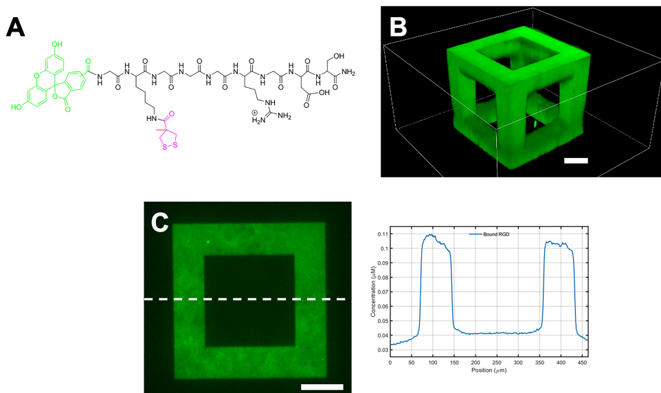
Figure S5.10 (A) Chemical structure of fluorescent RGD peptide ((fluorescein)GK(DT)GGGRGDS). (B) Representative images using confocal microscopy of the bound fluorescent RGD peptide throughout the DN hydrogel (5.0 mM SQ10SQ-DT /6.0 mM PEG 2-2 ) obtained via 3D direct-laser writing (DLW). (C) Raw 2D confocal fluorescence image of bounded fluorescent RGD peptide ( left ) and a graph of the measured concentration versus the position along the dashed line ( right ), highlighting the difference of the patterned and un-patterned area. Scale bar: 100 μm.
