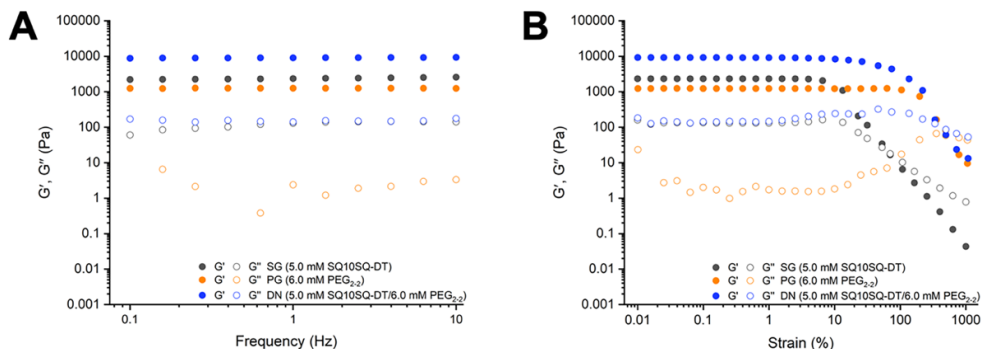
Figure S5.2 Averaged ( N = 3 ) (A) frequency (0.1-10 Hz) and (B) strain (0.01-1000%) sweeps of hydrogels with various compositions after 10 min UV irradiation ( \sim 10 mW/cm 2 , \lambda = 320 -500 nm, primary peak: 365 nm) at room temperature: SG (5.0 mM SQ10SQ-DT ), PG (6.0 mM PEG 2-2 ) and DN (5.0 mM SQ10SQ-DT /6.0 mM PEG 2-2 ). The frequency sweep experiment was performed at a fixed strain ( \gamma = 0.05\% ) and the strain experiment was collected at constant frequency ( f = 1.0 Hz).
