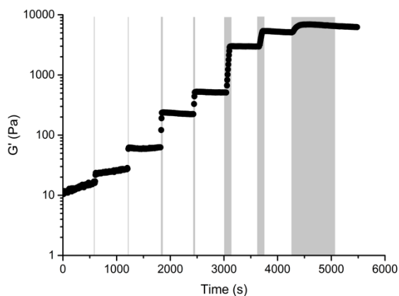
Figure S5.5 The averaged ( N = 2 ) time sweep experiment of DN hydrogel (5.0 mM SQ10SQ-DT /6.0 mM PEG 2-2 ) through step UV light irradiation (10 mW/cm 2 , wavelength: 320-500 nm, primary peak: 365 nm). The data was collected at a fixed frequency ( f = 1.0 Hz) and strain ( \gamma = 0.05\% ) at room temperature. The shaded area shows when the UV light was applied.
