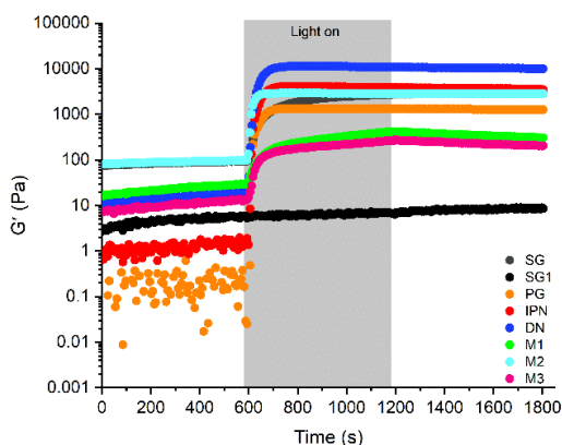
Figure S5.3 Averaged ( N = 3 ) time sweep experiment of various hydrogels after 10 min UV irradiation ( \sim 10 mW/cm 2 , \lambda = 320 -500 nm, primary peak: 365 nm) measured at a fixed frequency ( f = 1.0 Hz) and strain ( \gamma = 0.05\% ) at room temperature: (1) SG (5.0 mM SQ10SQ-DT ); (2) SG1 (5.0 mM SQ0SQ-DT ); (3) PG (6.0 mM PEG 2-2 ); (4) IPN (5.0 mM SQ0SQ-DT /6.0 mM PEG 2-2 ); (5) DN (5.0 mM SQ10SQ-DT /6.0 mM PEG 2-2 ); (6) M1 (5.0 mM SQ10SQ-DT /6.0 mM PEG 2-2 /no LAP ); (7) M2 (5.0 mM SQ10SQ-DT /3.0 mM PEGdiNB /1.0 mM LAP ); and (8) M3 (5.0 mM SQ10SQ-DT /3.0 mM PEGdiDT /1.0 mM LAP ). The shaded area shows when the UV light was applied.
