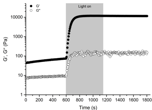
Figure S5.4 Averaged ( N = 2 ) time sweep experiment of DN hydrogel (10.0 mM SQ5SQ-DT /6.0 mM PEG 2-2 ) after 10 min UV irradiation ( \sim 10 mW/cm 2 , \lambda = 320 -500 nm, primary peak: 365 nm) measured at a fixed frequency ( f = 1.0 Hz) and strain ( \gamma = 0.05\% ) at room temperature. The shaded area shows when the UV light was applied.
