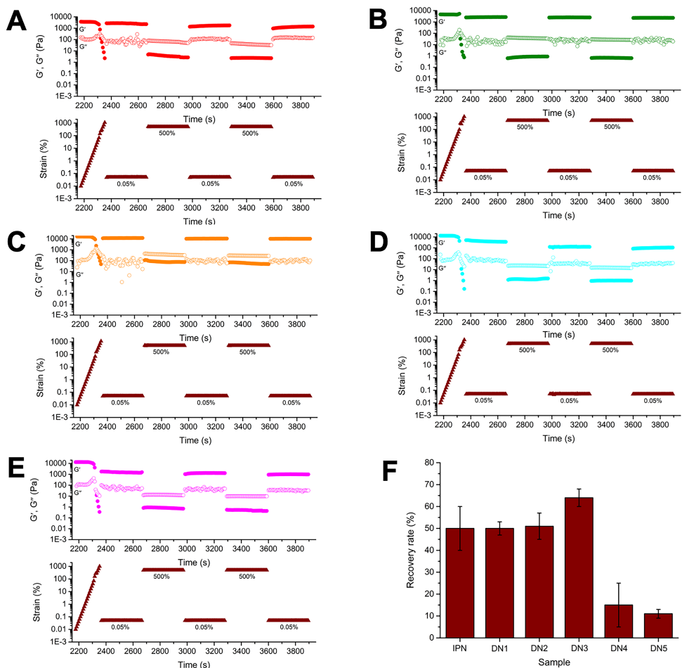
Figure S5.6 Averaged ( N = 3 ) strain experiment and step-strain measurement of various IPN and DN hydrogels after 10 min UV irradiation at a constant frequency ( f = 1.0 Hz): (A) IPN (5.0 mM SQ0SQ-DT /6.0 mM PEG 2-2 ); (B) DN1 (5.0 mM SQ10SQ-DT /3.0 mM PEG 2-2 ); (C) DN3 (5.0 mM SQ10SQ-DT /12.0 mM PEG 2-2 ); (D) DN4 (5.0 mM SQ10SQ-DT /4.5 mM PEG 2-4 ) and (E) DN5 (5.0 mM SQ10SQ-DT /3.0 mM PEG 4-4 ). (F) The averaged ( N = 3 ) storage recovery rate of various IPN and DN hydrogels. DN2: 5.0 mM SQ10SQ-DT /6.0 mM PEG 2-2 . For all measurements, UV irradiation condition: \sim 10 mW/cm 2 , wavelength: 320-500 nm, primary peak: 365 nm. Error bars were calculated according the average of independent repeat measurements ( N = 3 ).
