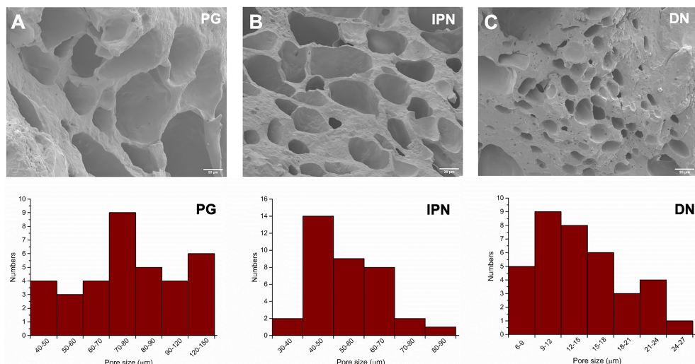
Figure S5.9 SEM images of various hydrogel systems (A) PG: 6.0 mM PEG 2-2 ; (B) IPN: 5.0 mM SQ 10 SQ-DT /6.0 mM PEG 2-2 ; (C) DN: 5.0 mM SQ 10 SQ-DT /6.0 mM PEG 2-2 and also their relative distribution of pore size. The pore size was measured from the SEM images using the Image J software. Scale bar: 20 μm.
