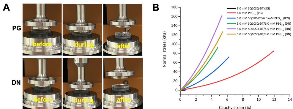
Figure 5.3 (A) Optical images illustrating the different states of hydrogels PG (6.0 mM PEG 2-2 ) and DN (5.0 mM SQ10SQ-DT/6.0 mM PEG 2-2 ) after 10 min UV irradiation ( \sim 10 mW/cm 2 , wavelength: 320–500 nm, primary peak: 365 nm) before/during/after the force experiments using rheology. (B) The averaged ( N = 3 ) normal stress-cauchy strain curves of different hydrogel samples (SG, PG, IPN and DN).
