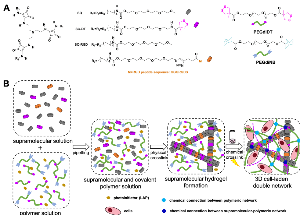
Figure 5.1 (A) Chemical structure of squaramide based supramolecular monomers ( SQ , SQ-DT and SQ-RGD ) and PEG-based polymeric monomers ( PEGdiDT and PEGdiNB ); (B) Schematic illustration for the preparation of 3D cell-laden supramolecular and covalent polymer based double networks, which follow three general steps and use UV irradiation (1-10 min, \sim 10 mW/cm 2 , 365-375 nm) to initiate covalent bond formation.
