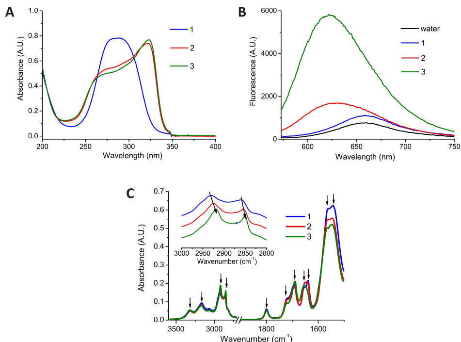
Figure 2.3 (A) UV-Vis spectra of molecules 1-3 in deionized water ( 1.5 \times 10^{-5} M). (B) Solutions of Nile Red ( 1.0 \times 10^{-6} M, Ex. 550 nm, Em. 560-750 nm) in deionized water and in the presence of 1-3 ( 1.5 \times 10^{-5} M). (C) FTIR spectra of samples 1-3 in the solid state (samples lyophilized from deionized water (3.1 mM), arrows highlight peaks considered).
