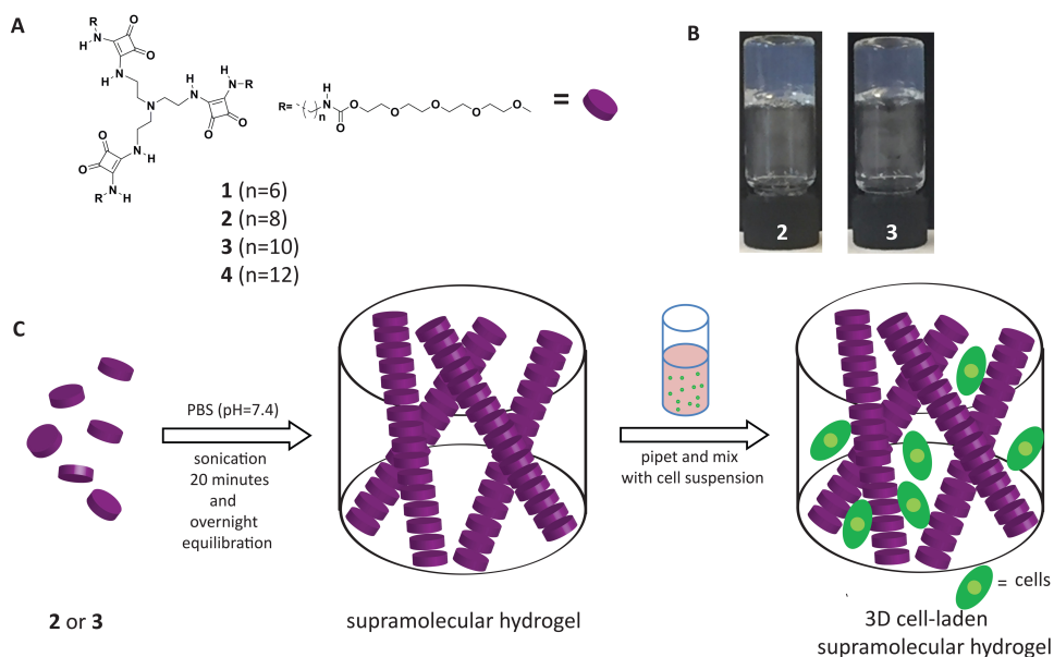
Figure 2.1 (A) Tripodal squaramide-based monomers 1-4 with varied alkyl chain lengths ( n = 6, 8, 10, 12 ). (B) Gel inversion test of squaramide-based materials above the CGC: 2 (5.6 mM) and 3 (3.1 mM) in deionized water. (C) Supramolecular hydrogel preparation and 3D cell seeding strategy.
