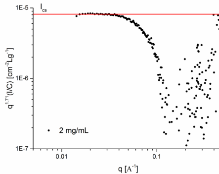
Figure S2.9 I_{cs}(q) determination plot of the scattering profile in Figure 2.2F . The I_{cs}(q) plateau ( 0.0143 \leq q \leq 0.0383 \text{ \AA}^{-1} ) is indicated by a red line.
