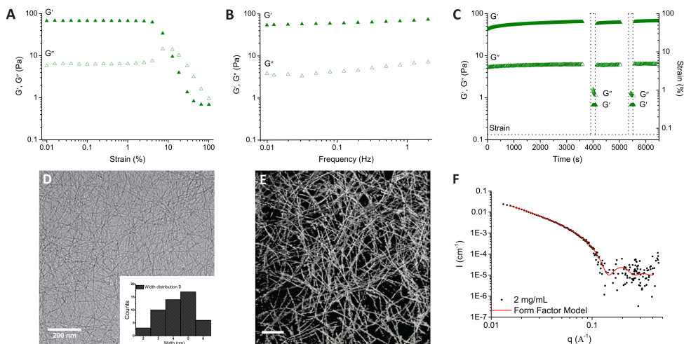
Figure 2.2 Oscillatory rheology measurements of the hydrogel 3 (3.1 mM) in PBS (pH = 7.4) at 37 °C: (A) Amplitude sweep ( f = 1 Hz). (B) Frequency sweep ( \gamma = 0.05\% ). (C) Step strain measurements ( f = 1 Hz), the absence of data before the application of high strain is due to the acquisition of a frequency sweep (from 0.01 to 2 Hz, \gamma = 0.05\% ). (D) Cryo-TEM image of a hydrogel 3 (3.1 mM). Insert: Histograms of width distribution of the fibres for a sample size of N = 50 . (E) Cryo-electron tomography image of a hydrogel of 3 (3.1 mM). Scale bar: 200 nm. (F) Small-angle X-ray scattering profiles of fibers 3 collected at a concentration of 2 mg mL -1 . Black dots represent experimental data; red line represents fit with a form factor for flexible cylinders.
