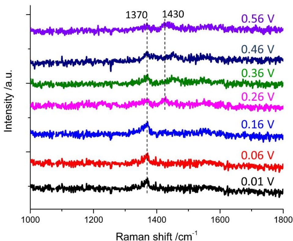
Figure 7. SERS spectrum of 1 mM of NPTS in 0.1 M \text{H}_2\text{SO}_4 on polycrystalline gold at different potentials from 0.01 to 0.56 V, see bands at 1370 and 1430 \text{ cm}^{-1} ; The full spectrum recorded between 0.01 to 1.06 V is shown in Fig. B9
