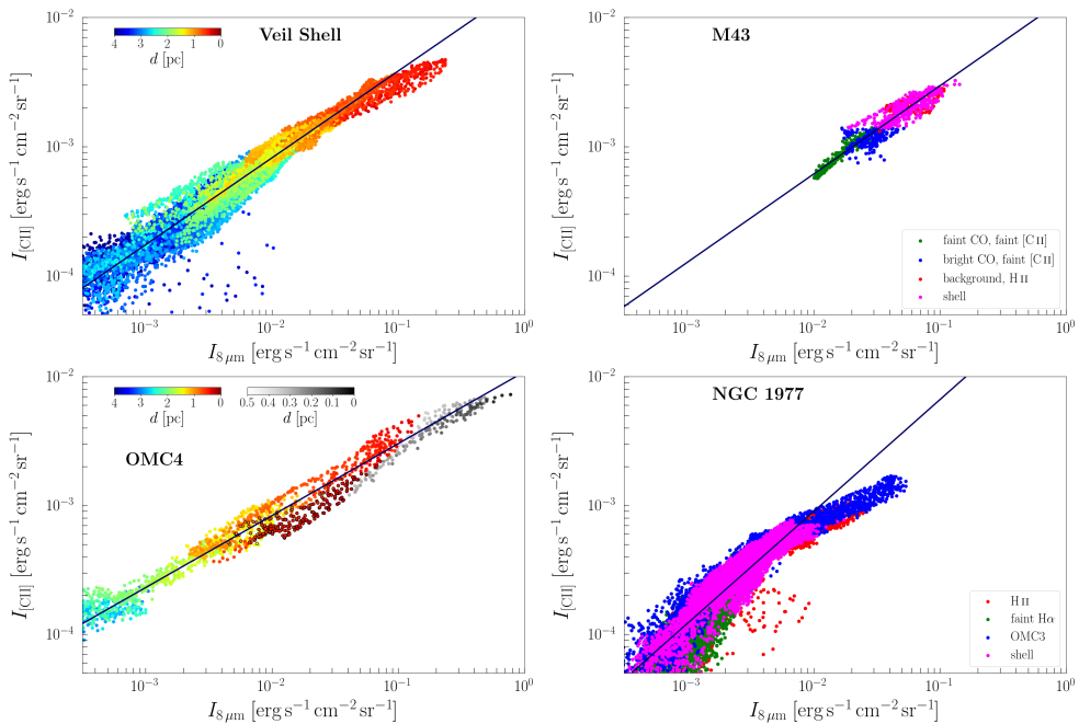
Figure 6.10: [C II] intensity versus IRAC 8 \mu\text{m} intensity in M42 (top left: Veil Shell, bottom left: OMC4 with OMC1 (in grey scale; black-edged red points lie to the west of Orion S)), M43 (top right) and NGC 1977 (bottom right). The color scale in M42 indicates the distance from \theta^1 Ori C. The division of M43 and NGC 1977 into the regions given in the legend is described in Section 6.3.2. The blue solid lines are the fits summarized in Table 6.4.
