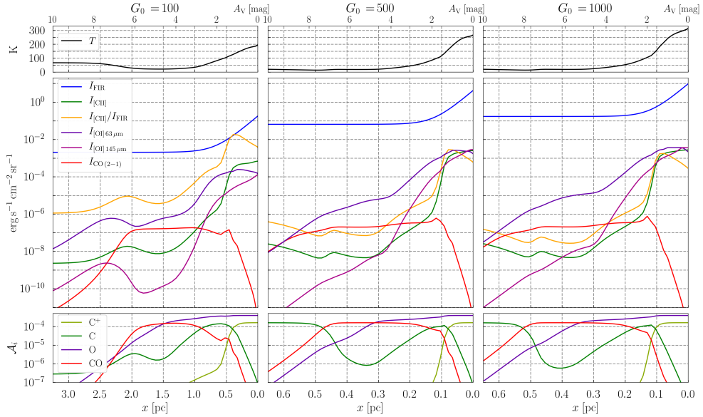
Figure 6.6: Results of our edge-on models described in Section 6.3.3 for incident FUV intensities of G_0 = 100, 500, and 1000 on physical scale, illuminated from the right. The panels show the gas temperature T (upper panels), I_{\text{FIR}}, I_{[\text{C II}]}, I_{[\text{C II}]/\text{FIR}}, I_{[\text{O I}] 63 \mu\text{m}}, I_{[\text{O I}] 145 \mu\text{m}}, and I_{\text{CO}(2-1)} (middle panels) and \text{C}^+, \text{C}, \text{O}, and \text{CO} fractional abundances (lower panels) versus physical scale. The gas densities are n_{\text{H}} = 2.0 \times 10^3 \text{ cm}^{-3}, 1.0 \times 10^4 \text{ cm}^{-3}, 1.0 \times 10^4 \text{ cm}^{-3} (left to right panels), and the respective line-of-sight depths are A_{\text{V,los}} = 3, 10, 10 .
