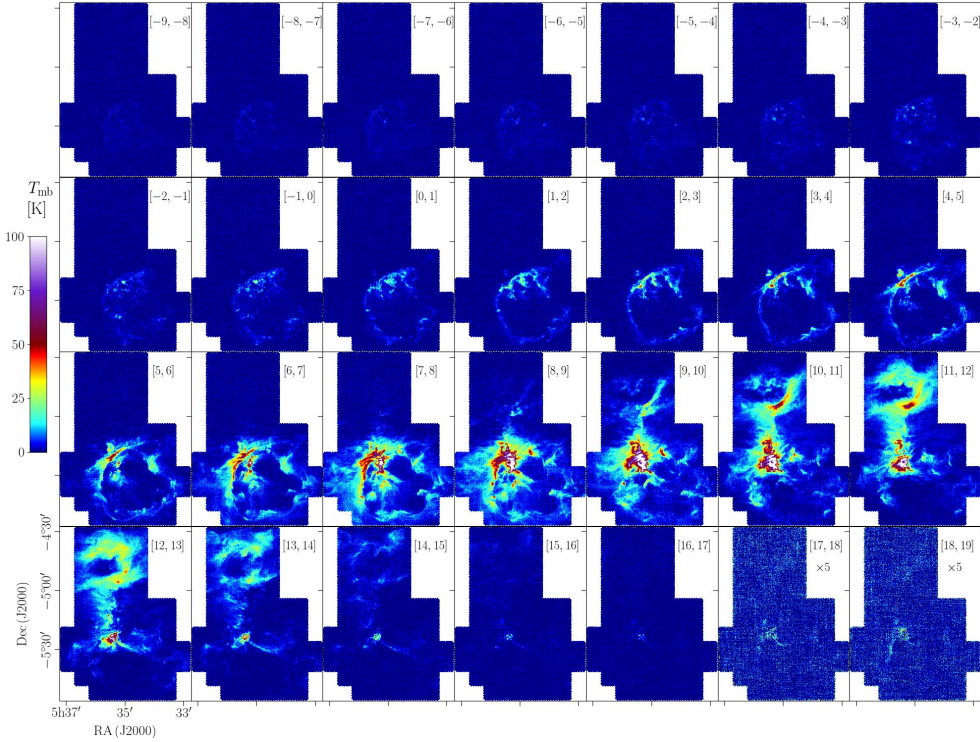
Figure 6.3: [C II] intensity per 1 \text{ km s}^{-1} channel in the range v_{\text{LSR}} = -9\text{--}19 \text{ km s}^{-1} . The intensities in the last two channels ( v_{\text{LSR}} = 17\text{--}19 \text{ km s}^{-1} ) contain ^{13}\text{C II} F = 2\text{--}1 emission and are multiplied by 5.
