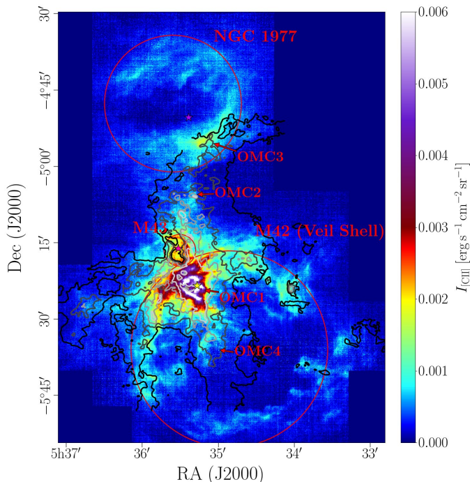
Figure 6.2: [\text{C II}] line-integrated intensity ( v_{\text{LSR}} = -10\text{-}20 \text{ km s}^{-1} ) from Orion A at its native resolution with CO(2-1) line-integrated intensity ( v_{\text{LSR}} = -10\text{-}20 \text{ km s}^{-1} , coverage not complete, cf. Paper I) in contours (from black to light grey: 1, 2, 3, 4 \times 10^{-6} \text{ erg s}^{-1} \text{ cm}^{-2} \text{ sr}^{-1} ). The red circles delineate the three distinct shells of M42, M43, and NGC 1977. The stars indicate the most massive stars within each region: \theta^1 Ori C (yellow) in M42, NU Ori (pink) in M43, and 42 Orionis (purple) in NGC 1977. Arrows indicate the positions of the four molecular cores OMC1-4 along the Integral-Shaped Filament.
