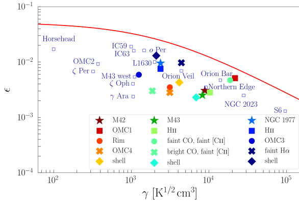
Figure 6.22: The average photoelectric heating efficiency \epsilon , equated as cooling efficiency [C\text{II}]/\text{FIR} , in M42, M43, and NGC 1977, divided into the previously defined subregions, as function of the ionization parameter \gamma = G_0 T^{1/2}/n_e . OMC1 includes [O\text{I}] cooling, but excludes the BN/KL region and Orion S. Parameters for Orion A are given in Table 6.7. The photoelectric heating efficiency in PDRs and diffuse sight lines from the literature is plotted as open blue squares (cf. Fig. 9 in Paper I). Data for the diffuse ISM are taken from Gry et al. (1992) and van Dishoeck & Black (1986), data of NGC 2023 are from Hollenbach & Tielens (1999), data for the Horsehead and L1630 are from Pabst et al. (2017), data for IC 59 and IC 63 are from Andrews et al. (2018), data for the Orion Bar, S6, M43 west, and OMC2 are from Herrmann et al. (1997), and data for the Orion Veil are from Salas et al. (2019). The red curve is the theoretical prediction of Eq. 43 by Bakes & Tielens (1994).
