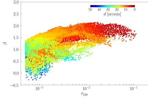
Figure 6.32: Dust optical depth \tau_{160} (> 5 \times 10^{-4}) versus grain emissivity index \beta ( \rho \simeq 0.32 ). Colors code the distance from \theta^1 Ori C.
