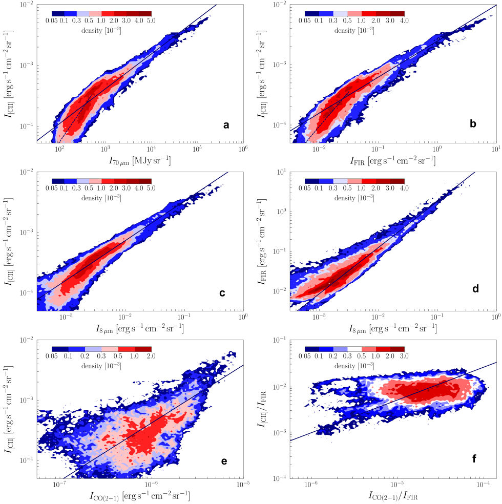
Figure 5.3: Correlations of all map points as point-density plots: a ) [C II]-70 \mu\text{m} , b ) [C II]-FIR, c ) [C II]-8 \mu\text{m} , d ) FIR-8 \mu\text{m} , e ) [C II]-CO(2-1), f ) [C II]/FIR-CO(2-1)/FIR. The regression curve with parameters of Table 5.1 is drawn in the respective panels (solid lines; dashed lines in panels a and b are the regression curves in the low-intensity regime).
