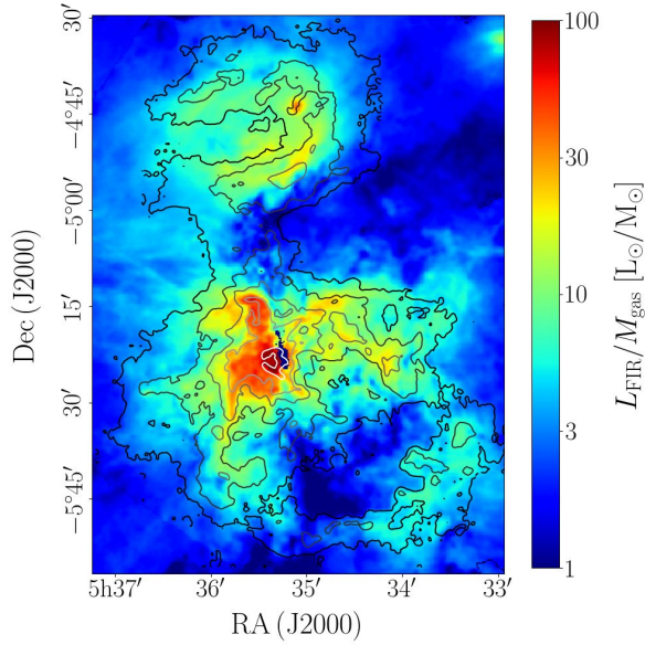
Figure 5.6: Spatial distribution of L_{\text{FIR}}/M_{\text{gas}} in Orion A with [C II] line-integrated intensity in contours (from black to white: 2, 5, 10, 20, 50 \times 10^{-4} \text{ erg s}^{-1} \text{ cm}^{-2} \text{ sr}^{-1} ).
