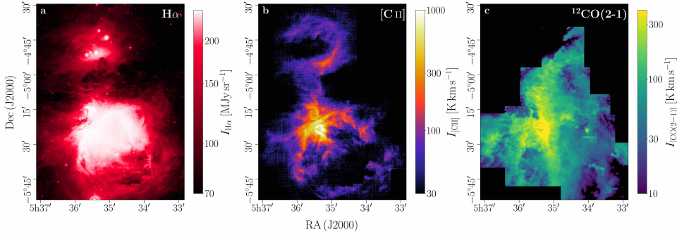
Figure 4.1: Overview of the Orion Nebula (M42), M43, and NGC 1773, 1775, and 1777 in different wavelengths. Left: DSS2 H\alpha emission (ESO Archive). Center: [C\ II] line-integrated emission (Pabst et al. 2019). Right: Line-integrated ^{12}CO(2-1) emission (Berné et al. 2014; Goicoechea et al. 2020). H\alpha emission stems from the ionized gas ( T \sim 10^4 K), the [C\ II] line is emitted by mostly neutral gas ( T \sim 100 K), whereas CO traces the molecular gas ( T \sim 30 K). M42 and M43 have a substantial amount of molecular gas in the background, while NGC 1777 seems to be devoid of it (the coverage of the CO map is not sufficient, however, see discussion of the expansion characteristics below). All three regions comprise ionized gas within their neutral limb-brightened shells.
