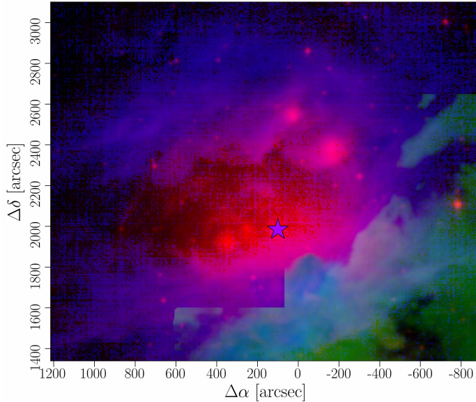
Figure 4.14: Three-color image of NGC 1977. Red is H\alpha emission from the ionized gas, green is line-integrated CO(2-1) emission from molecular gas (coverage only in OMC3), and blue is the [C II] line-integrated intensity, tracing the neutral gas.
