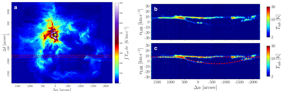
Figure 3.2: Position-velocity diagrams of the [C II] emission along selected cuts across the Veil. a) The Veil bubble in the integrated intensity of the 1.9-THz [C II] emission. The red lines delineate the region over which the spectra were collapsed to produce the east-west cut shown in b and c. The origin (yellow star) corresponds to the position of \theta^1 Ori C: right ascension RA(J2000) = 5h 35min 16.46s and declination dec.(J2000) = -5^\circ 23' 22.8'' ). The orange star indicates the position of an unrelated star, \theta^2 Ori A: RA(J2000) = 5h 35min 22.90s and dec.(J2000) = -5^\circ 24' 57.82'' . b) Position-velocity diagram of the [C II] emission in the east-west cut indicated in a. The velocity shown is measured in the frame of the local standard of rest. Other horizontal and vertical cuts yield similar diagrams (Fig. 3.10). c) A simple model of a spherical half-shell expanding at a constant velocity of 13 \text{ km s}^{-1} (red dashed lines) is fitted to the data in b. All of the observational position-velocity diagrams are in good agreement with this simple model.
