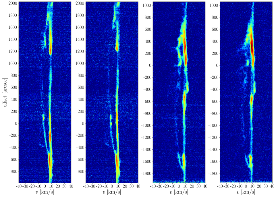
Figure 3.10: Four exemplary position-velocity diagrams of the [C II] emission from selected cuts across the Veil. Each position- velocity diagram exhibits a clear arc structure extending over about 2,500'' , which corresponds to the expanding Veil shell (C.P. et al., manuscript in preparation). The left (right) two panels are cuts along the horizontal (vertical) axis.
