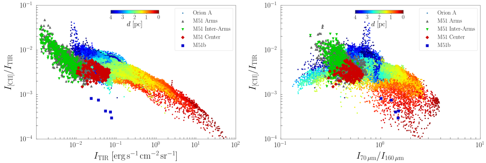
Figure 5.7: Left: [C II]/TIR intensity ratio versus TIR intensity in M51 and the Orion Nebula with M43. Right: [C II]/TIR intensity ratio versus PACS 70 \mu\text{m} over 160 \mu\text{m} intensity ratio in M51 and the Orion Nebula with M43. Fig. 1 in Pineda et al. (2018) shows the mask used to divide the M51 map into the four separate regions displayed here. Colors in Orion indicate distance from Trapezium stars as before (see colorbar).
