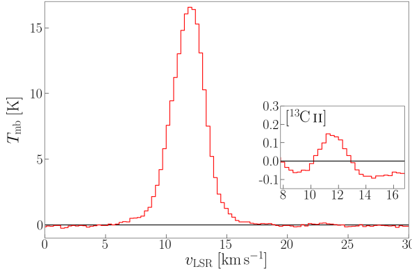
Figure 4.15: Average [C II] spectrum towards [C II]-bright shell of NGC 1977 (without OMC3). The inlaid panel shows the (smoothed) residual of the spectrum, in the systemic velocity of the ^{13}\text{C II} F = 2-1 line, after subtracting the ^{12}\text{C II} fit. The ^{12}\text{C II} component can be approximated by a Gaussian with T_P \simeq 16.5 \pm 0.1 K, v_P \simeq 12.0 \pm 0.1 km s ^{-1} , \Delta v_{\text{FWHM}} \simeq 3.2 \pm 0.1 km s ^{-1} ; the ^{13}\text{C II} F = 2-1 component is fitted by a Gaussian with T_P \simeq 0.21 \pm 0.03 K, v_P \simeq 11.8 \pm 0.2 km s ^{-1} , \Delta v_{\text{FWHM}} \simeq 2.1 \pm 0.5 km s ^{-1} .
