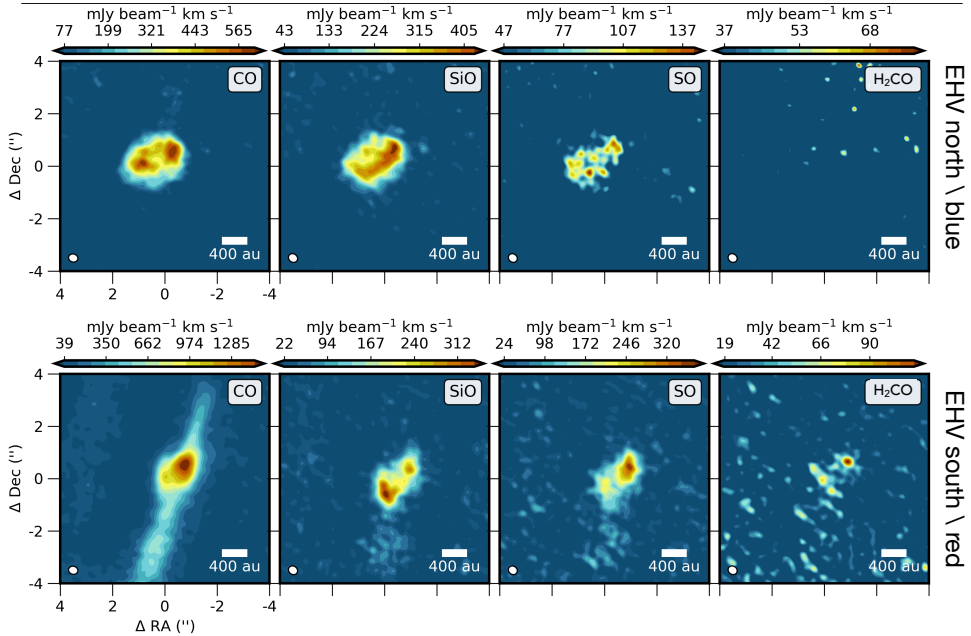
Figure 5.7: Zoom-in on molecular bullets from the SMM3 jet (see Fig. 5.6). CO, SiO, SO, and H 2 CO molecular transitions are presented. Top: Norther/blue-shifted bullet. Moment 0 maps are integrated from -60 to -40 km s -1 w.r.t v_{\text{sys}} . The map center is offset from the SMM3 continuum center by (-3'7, +10'3). Bottom: Southern/redshifted bullet. Moment 0 maps are integrated from 20 to 40 km s -1 . The map center is offset from the SMM3 continuum center by (+2'7, -7'').
