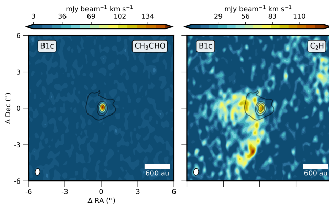
Figure 5.16: Emission maps of an example COM and hydrocarbon toward B1-c. Left: CH_3CHO moment 0 map, Right: C_2H moment 0 map; both integrated from -2 to 2 km\ s^{-1} w.r.t v_{sys} .
