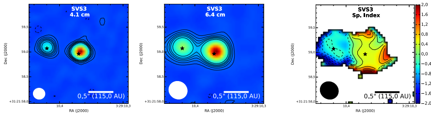
Figure 2.C.3: Maps of SVS3 system centered on a SVS3-B component. From left to right: 4.1 cm, 6.4 cm and spectral index map.
