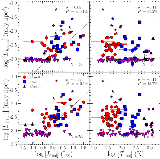
Figure 2.2: Luminosity at 4.1 cm (bottom) and 6.4 cm (top) compared with bolometric luminosity (left) and temperature (right). Spearman’s rank correlation coefficient and probability of no correlation is shown in the top-right corner. Sources with resolved radio jets are marked as stars and upper limits as magenta triangles.
