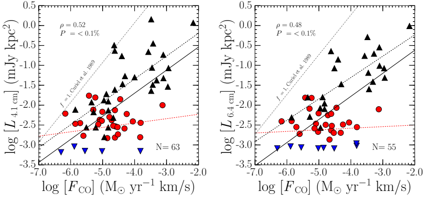
Figure 2.9: Radio luminosity at 4.1 cm (left) and 6.4 cm (right) plotted against outflow force from CO observations. Red and black dashed lines shows linear fits to the VANDAM and Shirley et al. (2007) samples respectively. Solid lines represent fits to the merged sample. Black dash-dot line represent the expected C-band fluxes from the outflow force alone, assuming 100% efficiency following Curiel et al. (1989). This line correspond to the maximum C-band fluxes that can be produced from the CO outflows.
