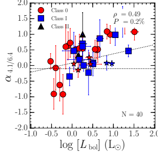
Figure 2.B.1: Left: Spectral index compared with bolometric luminosity with four outliers removed: Per-emb-14, EDJ2009-156, SVS13A2, L1448NW.
