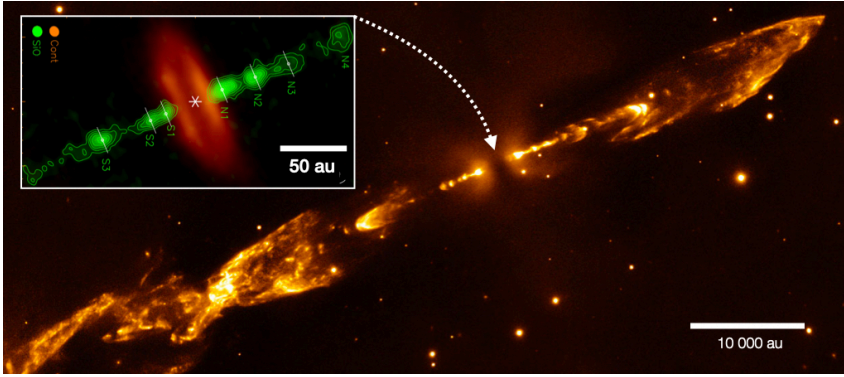
Figure 1.3: Image of the protostellar outflow toward HH212 protostar, through 2.12\ \mu\text{m} shocked \text{H}_2 observations with VLT (McCaughrean 1994). Inset shows the molecular jet seen in \text{SiO} 5–4 transition at 1.3 mm and the continuum emission from the disk at 1.3 mm (Lee et al. 2017).
