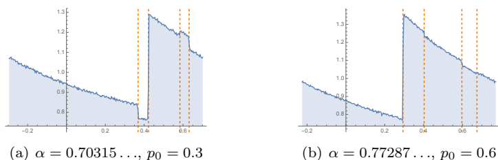
Figure 5.13: Numerical simulations of the invariant probability densities of the random continued fraction maps R_\alpha from Example 5.3.2. In (a) we take \alpha \in J_4 and p_0 = 0.3 and in (b) we have \alpha \in J_5 and p_0 = 0.6 . The dashed lines indicate the positions of the prematching points, i.e., the points in the orbits of \alpha and \alpha - 1 before the moment of matching.
