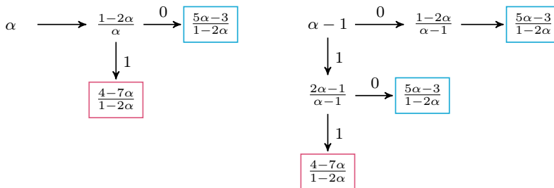
Figure 5.7: The first three elements in the orbits of \alpha and \alpha - 1 under the random continued fraction map R_\alpha for \alpha \in (\frac{\sqrt{10}-2}{2}, 2 - \sqrt{2}) . The digits above the arrows indicate which one of the maps T_{\alpha,0} or T_{\alpha,1} is applied. If there is no digit, then both maps yield the same orbit point. Orbit points in boxes with the same colour are equal.
