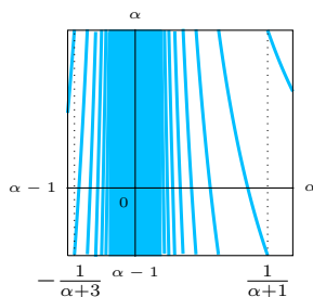
Figure 1.9: Example of T_\alpha for \alpha = \frac{7}{10} .
