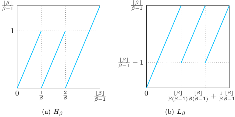
Figure 1.4: Example of the greedy and lazy \beta -transformations, for \beta = 2.39 .
