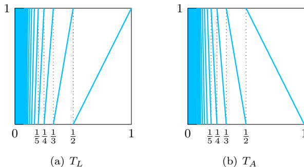
Figure 1.6: The standard and alternating Lüroth maps, respectively.
