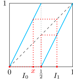
Figure 1.2: The doubling map D and in red the orbit of x = 3/8 .
