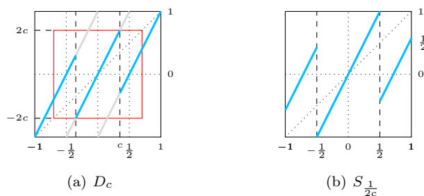
Figure 5.10: The maps D_c and S_{\frac{1}{2c}} for c = \frac{7}{20} . The grey lines indicate the remainder of the maps x \mapsto 2x+1 , x \mapsto 2x and x \mapsto 2x-1 . The red box in (a) shows the attractor of the map D_c .
