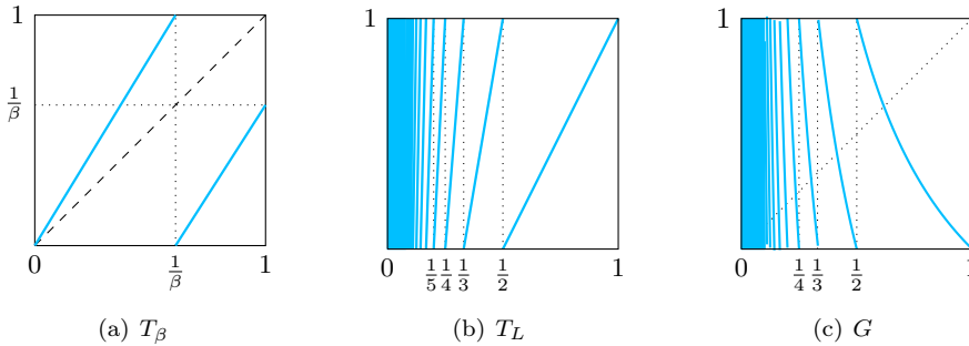
Figure 1.1: Classical examples of interval maps producing number expansions.
