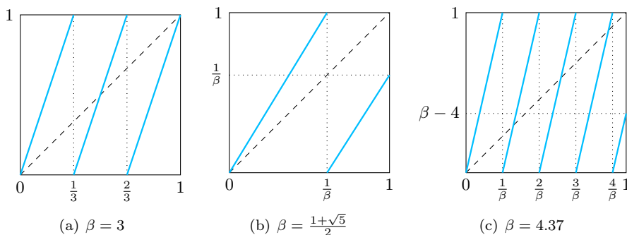
Figure 1.3: Examples of \beta -transformations T_\beta .
