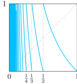
Figure 1.7: The Gauss map G .
