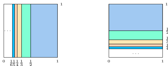
Figure 1.8: The action of the map S on the domain [0, 1]^2 of the natural extension for the Gauss map G . Areas on the left are mapped to areas on the right with the same colour.
