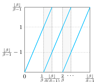
Figure 1.5: The random \beta -transformation for \beta = 2.39 .
