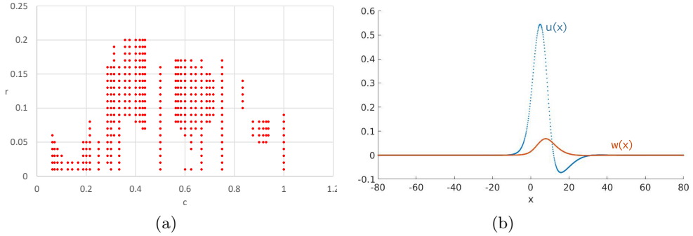
Figure 4.1: (a) Numerical computations of the pairs (c, r) for which travelling wave solutions to the system (4.2.40) exist. We emphasize that there may be parameter values where we could not find a solution, but where a solution exists nonetheless. These simulations clearly show that the relationship r(c) is multi-valued. (b) A plot of one of the travelling waves found in this numerical procedure with r = 0.11 and c = 0.3125 .
