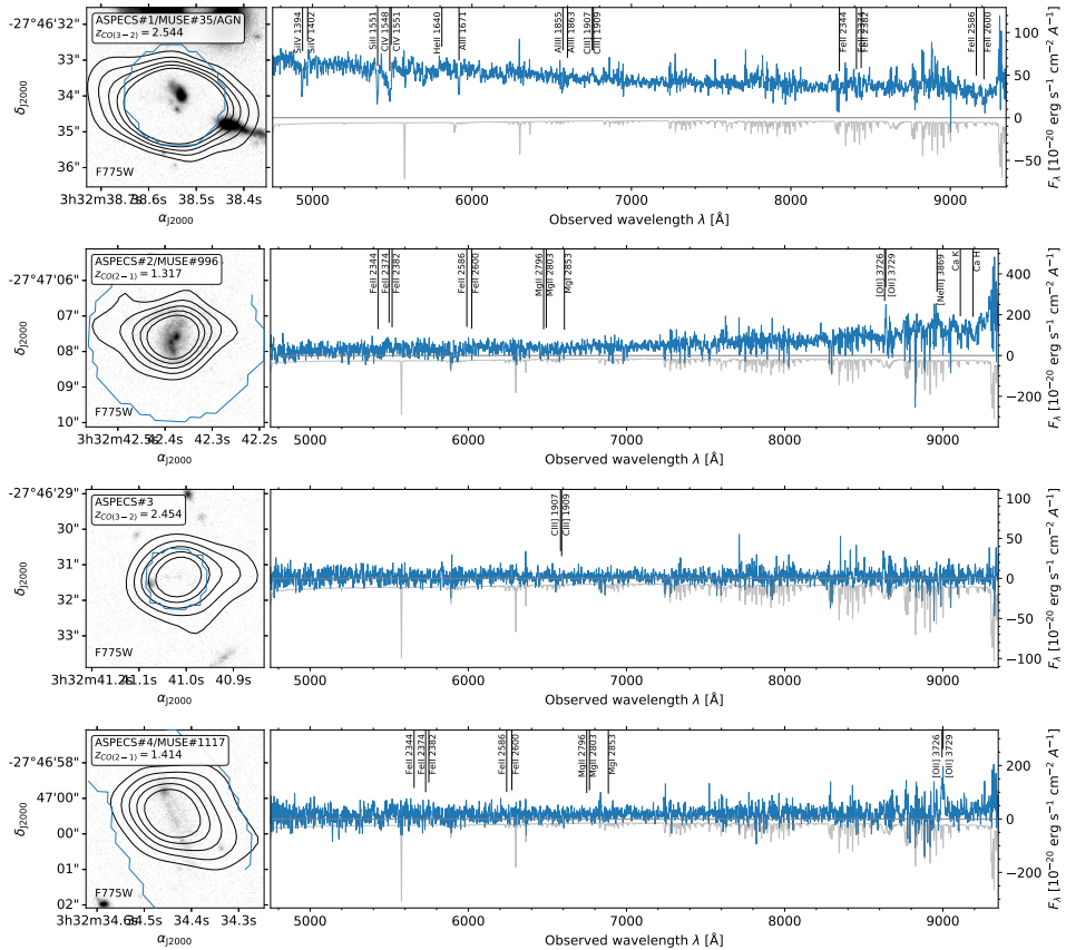
Figure 3.13: MUSE spectroscopy of the ASPECS-LP sources. Left: HST /F775W cutout. The colored contour(s) mark the region of the spectral extraction(s), defined by convolving the MUSE PSF with the HST segmentation map (see Inami et al. 2017 for details), or a fixed 0.8'' aperture (in the case of a new extraction; #3, #7, #9, #13). The black contours indicate the CO emission from \pm[3, \dots, 11]\sigma in steps of 2\sigma . Right: MUSE spectrum ( 1.5 \text{ \AA} Gaussian smoothing) extracted over the marked region. The 1\sigma uncertainty on the spectrum is shown by the gray line in the direction of negative flux (for clarity), and is largest around skylines. The (expected) positions of different spectral features are annotated; this does not indicate that the feature is also detected. Spectra and lines of nearby or blended sources are shown in red.
