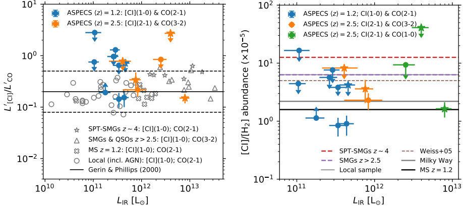
Figure 4.11: Left: L_{[C I]}/L'_{CO} ratio for [C I]( ^3P_1 \rightarrow ^3P_0 ) over CO(2-1) (blue) and [C I]( ^3P_2 \rightarrow ^3P_1 ) over CO(3-2) (orange), where stars indicate X-ray AGN. We compare the observed ratios to SPT-SMGs at z = 4 (Bothwell et al., 2017), SMGs at z \geq 2.5 (Walter et al., 2011; Alaghband-Zadeh et al., 2013), main-sequence galaxies at z = 1.2 and local galaxies, as compiled by Valentino et al. (2018), and the average ratio and scatter in the local sample from Gerin & Phillips (2000). Overall, the ratios broadly agree with the spread found for previous samples of star-forming galaxies. Right: atomic carbon abundance in the ASPECS galaxies. The H 2 mass was derived from CO(2-1) (assuming r_{21} = 0.75 \pm 0.11 ) and CO(1-0) or CO(3-2) (assuming r_{31} = 0.77 \pm 0.14 ), with \alpha_{CO} = 3.6 M_{\odot} (K \text{ km s}^{-1} \text{ pc}^2)^{-1} , for the galaxies detected in [C I](1-0) and [C I](2-1) respectively. We compare our measurements to the abundances for different galaxy types (excluding active galaxies), converted to a common \alpha_{CO} by Valentino et al. (2018). On average we find [C I] abundances similar to the Milky Way (Frerking et al., 1989) and the star-forming galaxies from Valentino et al. (2018) (who assumes a galaxy-specific \alpha_{CO} , which is 3.0 on average, and r_{21} = 0.84 ), with higher abundances at \langle z \rangle = 2.5 compared to \langle z \rangle = 1.2 . Note that the higher abundances in the submillimeter galaxies from literature are partly driven by the assumed lower \alpha_{CO} in these systems.
