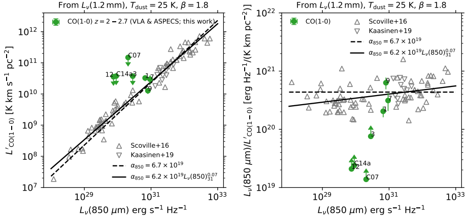
Figure 4.9: Rest frame luminosity at 850 \mu\text{m} compared to the CO(1-0) luminosity ( left ) and the ratio of L_V(850 \mu\text{m})/L'_{\text{CO}(1-0)} ( right ). The CO(1-0) observations were taken with the VLA (Riechers et al., 2020) and are re-analyzed in this paper. Sources are indicated by the 3mm.ID (except 1mm.CO7 and 1mm.C14a). The black lines show the best fit empirical relations from Scoville et al. (2016, assuming both a constant and dust-luminosity dependent dust-to-gas conversion factor), while the gray triangles show their calibration sample as well as more recent observations from Kaasinen et al. (2019).
