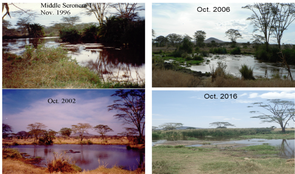
Fig. 10. Sequential photographs from 1996 to 2016, in the dry season, of the same waterhole in the Seronera River. The water hole is silting and this affects the dry season water availability for wildlife.
