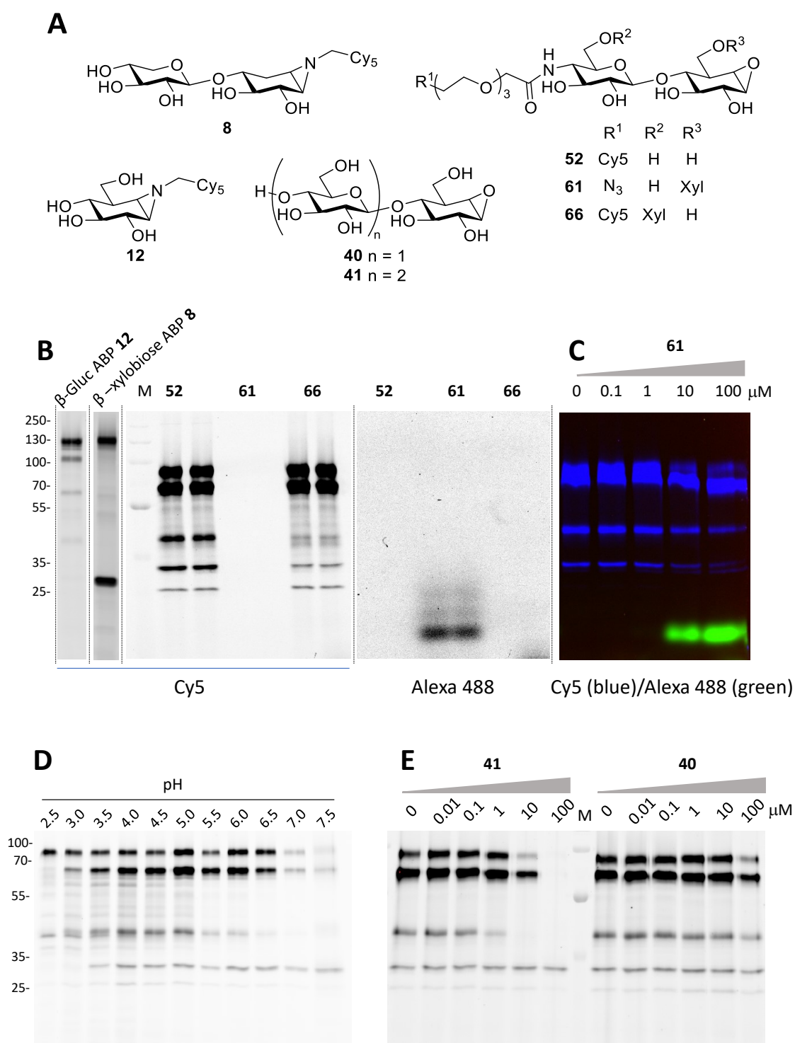
Figure 2.5 | Labeling of Aspergillus niger secretomes in Mcllvaine buffer pH 5.0 or the indicated pH. A) Structures of probes used in this figure. B) Labeling with probes with different recognition elements shows a different pattern. C) Incubation with various concentrations of GX 61 followed by labeling with GG 52 and ligation with Alexa 488 alkyne shows Alexa 488 labeling is dependent on concentration of 61 . D) Labeling with GG 52 is pH dependent. E) Incubation with GGG ( 41 ) and GG ( 40 ) configured inhibitors impairs labeling with GG configured probe 52 .
