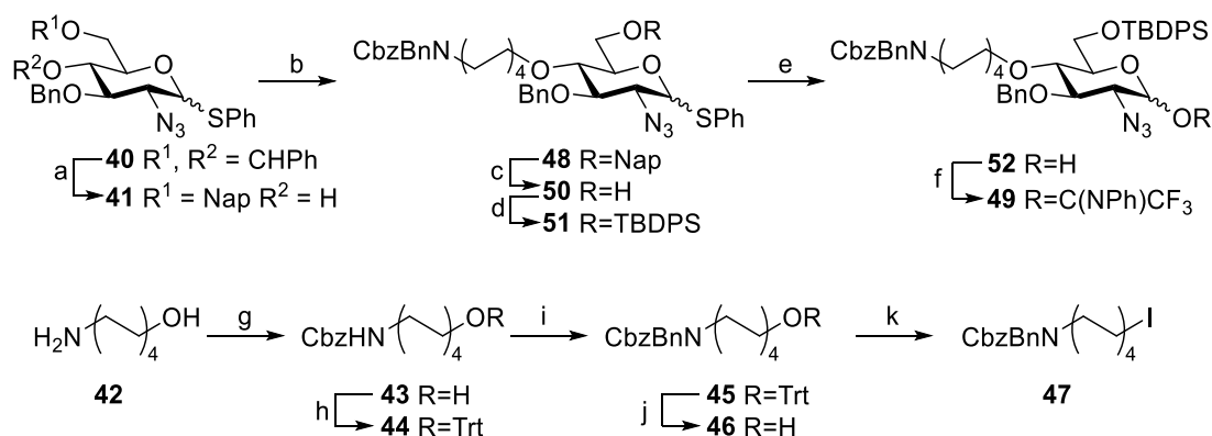
Scheme 3.5 | Reagents and conditions: a ) i. CSA, MeOH, DCE, 50°C; ii. NapBr, 2-aminoethyl diphenyl borinate, MeCN, 60°C, 93%. b ) 47 , NaH, DMF, 88%. c ) DDQ, DCM, MeOH, 72%. d ) TBDPSCl, imidazole, DMF. e ) NIS, acetone/H 2 O, DCM, 79%. f ) N -phenyl-trifluoroacetimidoylchloride, Cs 2 CO 3 , DCM, 94%. g ) CbzCl, NaHCO 3 , acetone/H 2 O, 88%. h ) TrtCl, Et 3 N, DMF. i ) BnBr, NaH, TBAI, DMF, 76% over 2 steps. j ) 3% TFA/H 2 O, DCM/MeOH, 84%; k ) PPh 3 , I 2 , imidazole, DCM, 97%.
