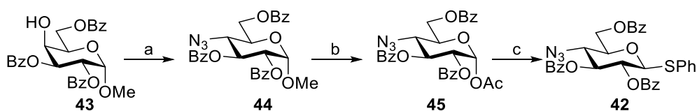
Scheme 2.4 | Reagents and conditions: a ) i. Tf_2O , pyr, DCM, -55^\circ C to rt; ii. NaN_3 , DMF, 80^\circ C , 90%. b ) Ac_2O , AcOH, H_2SO_4 . c ) HSPH, BF_3 \cdot Et_2O , DCM, 46% over 2 steps.
