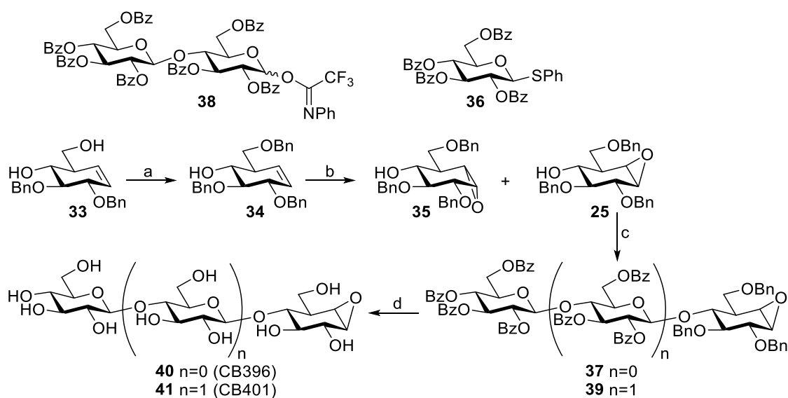
Scheme 2.3 | Reagents and conditions: a ) 2-aminoethyl diphenylborinate, KI, K_2CO_3 , BnBr, MeCN, 60^\circ C , 91%. b ) 1,1,1 trifluoroacetone, oxone, EDTA, NaHCO_3 , H_2O , MeCN, 0^\circ C , 52% ( 25 ) and 46% ( 35 ). c ) for 37 : 36 , NIS, TMSOTf, DCM, -30^\circ C to -10^\circ C , 53%. For 39 : 38 , TSMOTf, DCM, -15^\circ C to 0^\circ C , 45%. d ) i. NaOMe, MeOH; ii. H_2 , Pd(OH)_2/C , H_2O , MeOH, dioxane, for 40 quant., for 41 45%.
