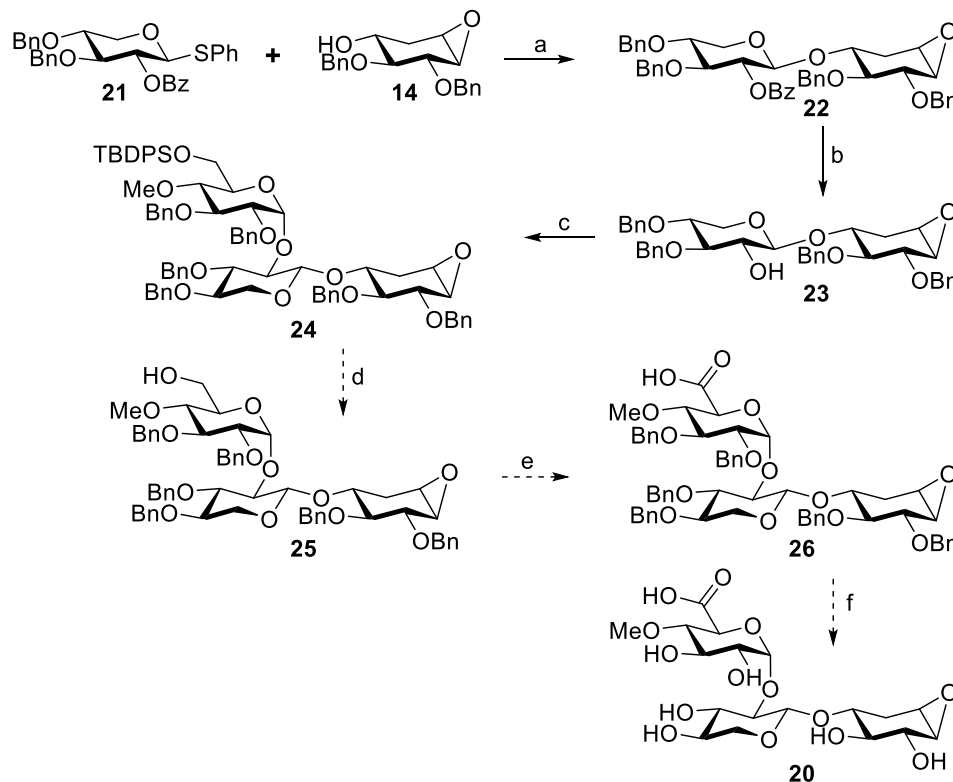
Scheme 5.3 | Reagents and conditions: a ) TMSOTf, NIS, DCM, -70°C to -50°C, 73%. b ) NaOMe, MeOH, DCM, 78%. c ) 10 , Tf 2 O, Ph 2 SO, TTBP, DCM, Et 2 O, -70 to -50°C, 30%. Proposed reagents and conditions: d ) 3HF·Et 3 N, THF. e ) TEMPO, BAIB, DCM, t -BuOH, H 2 O. f ) Na(s), t -BuOH, NH 3 , THF.
