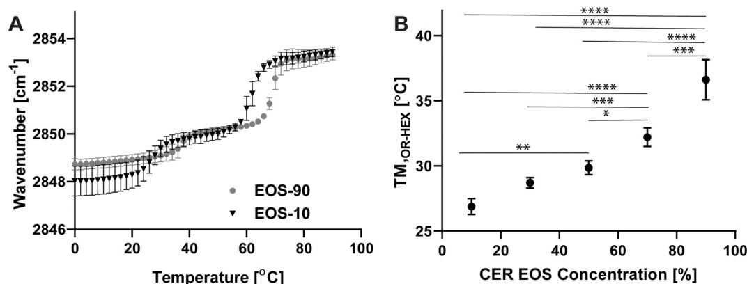
Fig. 3. The thermotropic response of the \nu_s\text{CH}_2 modes and midpoint temperatures of the orthorhombic-hexagonal phase transition ( T_{\text{M,OR-HEX}} ).
