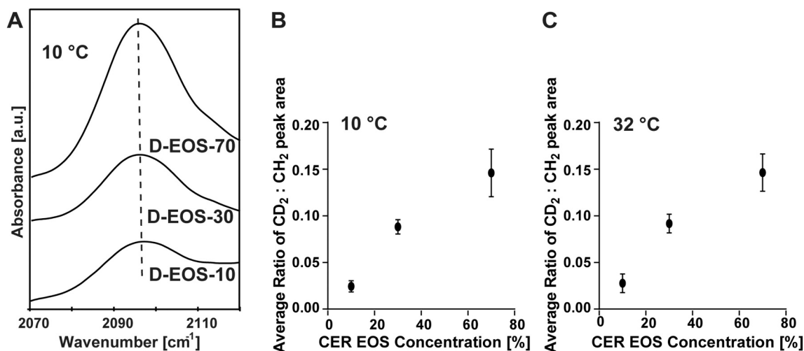
Fig. 6. Peak position of \nu_s\text{CD}_2 and peak area ratio of \nu_s\text{CD}_2 to \nu_s\text{CD}_2 .
