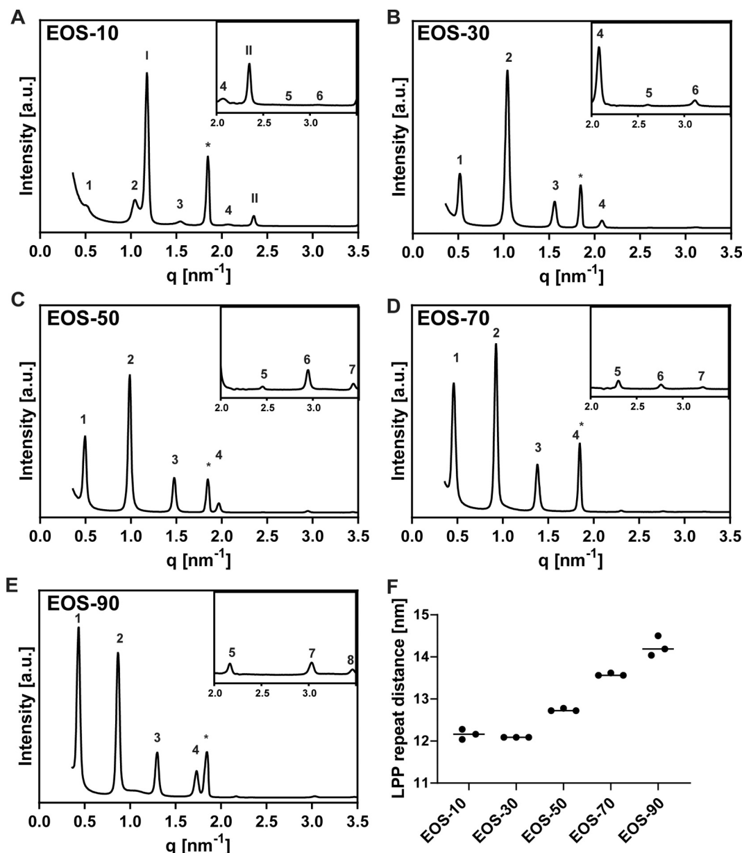
Fig. 7. X-ray diffraction profile of the lipid models.
