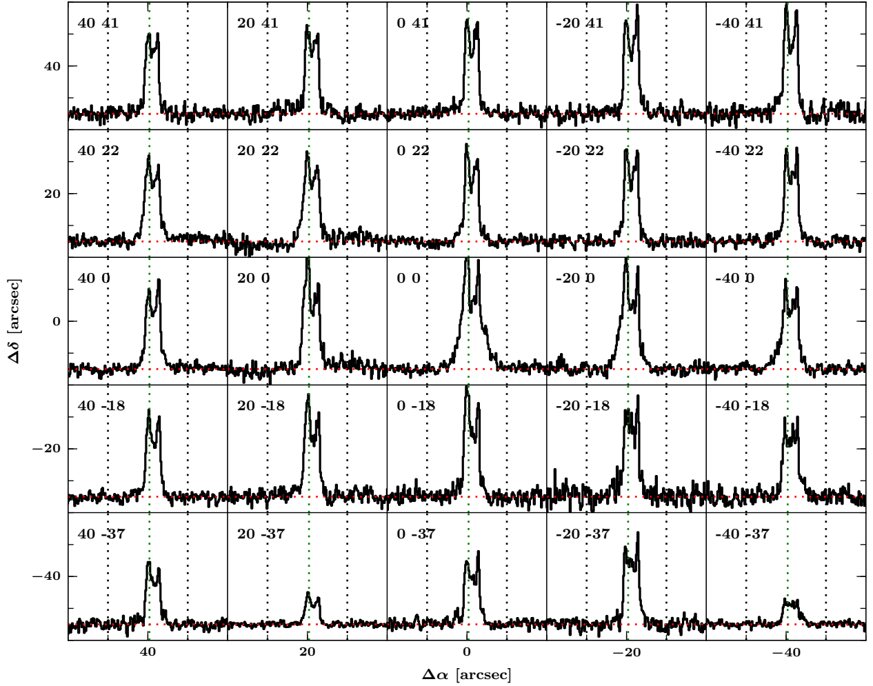
Fig. D.1. ^{12}\text{CO } J = 3-2 spectral map obtained with the JCMT from -5 \text{ km s}^{-1} to 15 \text{ km s}^{-1} and intensities from -0.5 \text{ K} to 3.5 \text{ K} . The vertical dotted lines show 0, 5.2, and 10 \text{ km s}^{-1} for guidance.
