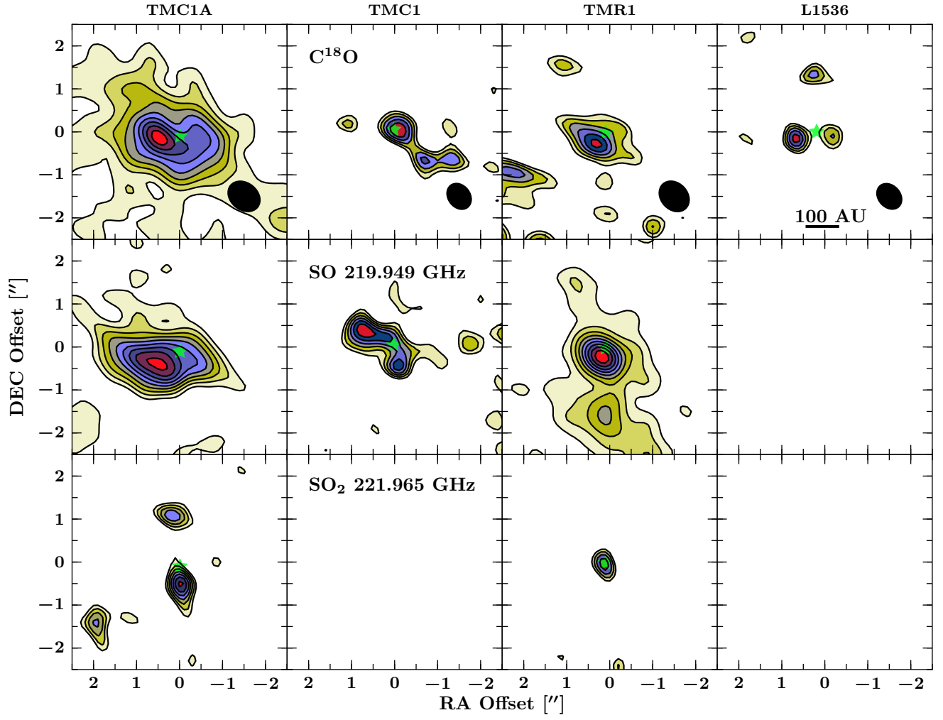
Fig. C.3. Moment 0 maps of \text{C}^{18}\text{O } J = 2-1 , \text{SO } 5_6-4_5 and \text{SO}_2 11_{1,1}-10_{0,0} toward all sources from the WideX data. The contours are drawn at 10% of the peak starting at 3\sigma . Green star indicates the continuum position and black ellipses show the synthesized beams.
