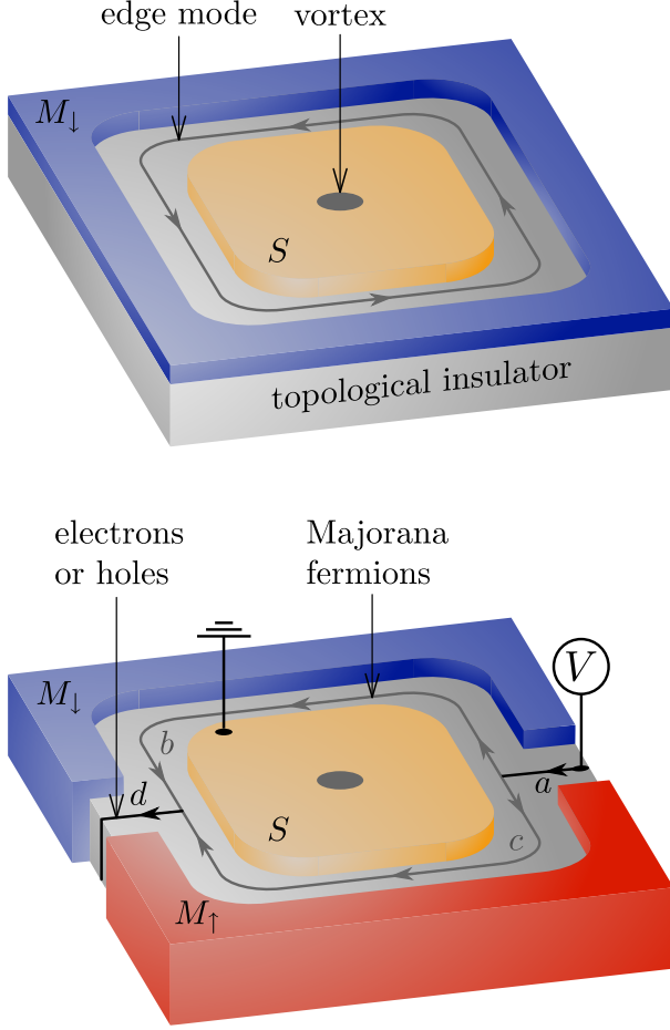
FIG. 1 (color online). Three-dimensional topological insulator in proximity to ferromagnets with opposite polarization ( M_\uparrow and M_\downarrow ) and to a superconductor ( S ). The top panel shows a single chiral Majorana mode along the edge between superconductor and ferromagnet. This mode is charge neutral, so it cannot be detected electrically. The Mach-Zehnder interferometer in the bottom panel converts a charged current along the domain wall into a neutral current along the superconductor (and vice versa). This allows for electrical detection of the parity of the number of enclosed vortices, as explained in the text.
