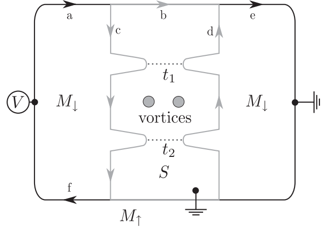
FIG. 2. Fabry-Pérot interferometer, allowing to measure the state of a qubit encoded in a pair of vortices. Black lines represent electron or hole modes at domain walls, gray lines represent Majorana modes at magnet-superconductor interface.
