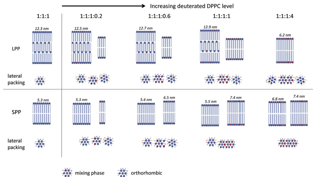
Fig. 6. A model of the induced changes in phase behaviour when increasing the DPPC level in lipids forming initial the long periodicity phase (LPP) or the short periodicity phase (SPP). The ratios provided are the ratios between CER (EOS/NS or NS): CHOL:FA24:DPPC. The red head-groups indicate perdeuterated DPPC. The blue head-groups refer to the SC lipids.
