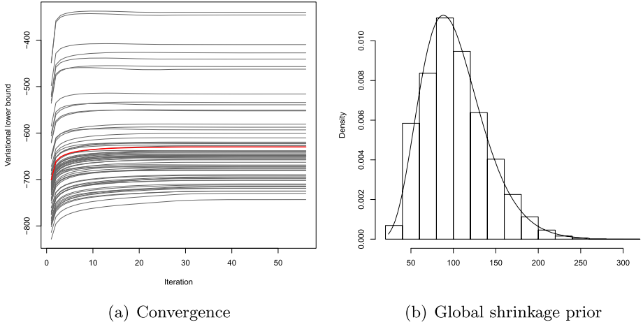
FIG. 1. Illustration of (a) the convergence of the variational algorithm and (b) the estimated global shrinkage prior on the breast cancer data set (P53 pathway). Figure (a) displays the variational lower bounds \mathcal{L}_j of each regression equation in the SEM as a function of iterations. The red continuous line represents the average lower bound. Figure (b) displays an empirical mixture of marginal posteriors of \tau_j^{-2} obtained by drawing 1000 samples from q_2^j(\tau_j^{-2}; \mathbf{y}_j) , \forall j . The continuous line represents the density of the estimated global shrinkage prior on \tau_j^{-2} , which corresponds to \mathcal{G}(7.404, 0.073) .
