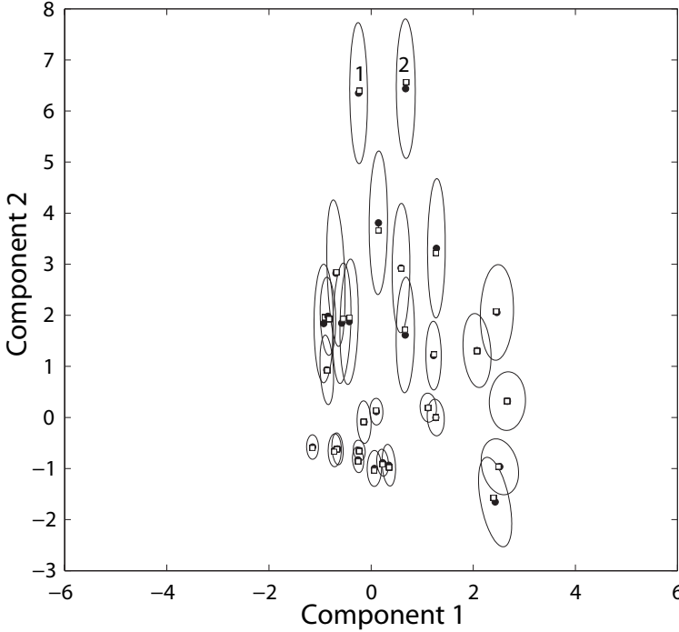
Figure 3.6: 90% confidence ellipses for the person scores from the recoded ORCE data. Black circles indicate the centroids of the bootstrap clouds. White squares represent the original person scores. The 2.5% (i.e., 15) largest confidence ellipses have been selected for display. In addition, a random selection of 15 other ellipses is displayed.
