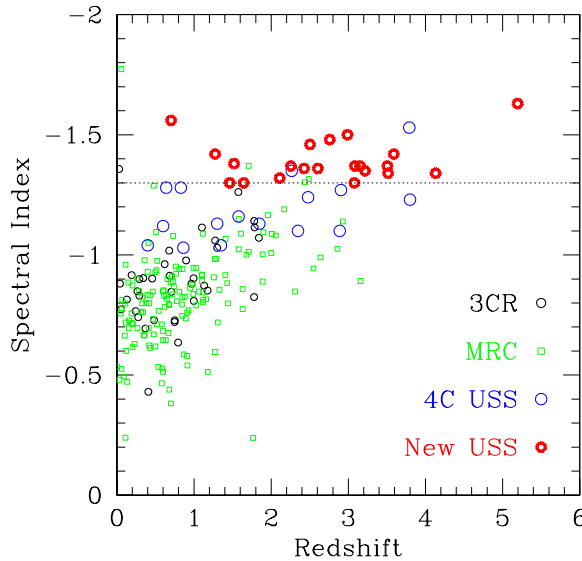
Figure 1.2: The correlation between spectral index and redshift seen for bright radio galaxies. Plot from De Breuck et al. (2000).
