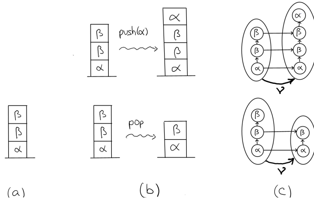
Figure 1: (a) Illustration of a pushdown configuration, (b) illustration of instances of the instructions \text{push}(\alpha) and \text{pop} , (c) two pair graphs corresponding to the instances of the instructions shown in (b).
