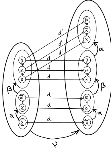
Figure 10: A pair graph for the instruction \text{push}(\alpha, \text{down}(\beta)) as implemented in the MSO graph storage type \bar{P}(\text{STACK}) .
