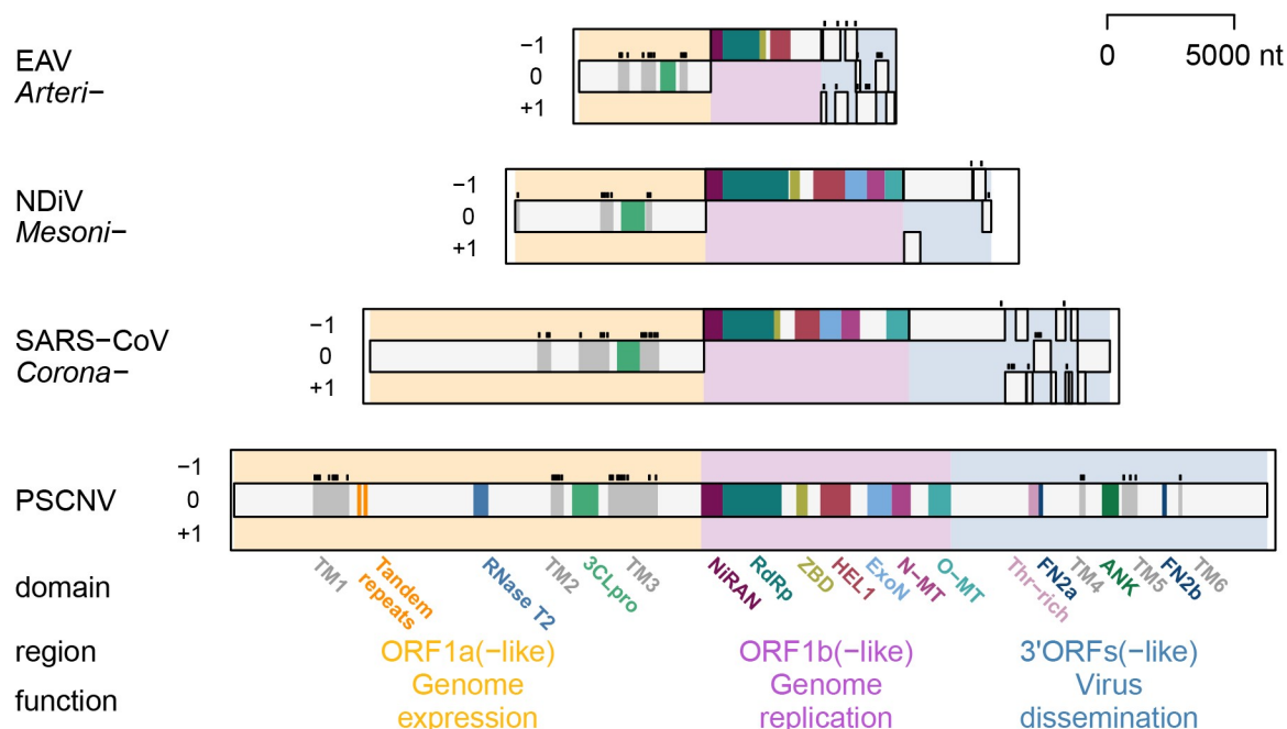
Fig 2. Genomes and proteomes of nidoviruses. ORFs and encoded protein domains in genomes of viruses representing three nidovirus families and PSCNV. The protein-encoding part of the genomes is split in three adjacent regions, which are colored and labelled accordingly. EAV, equine arteritis virus; NDiV, Nam Dinh virus; SARS-CoV (see S1 Table for details on these viruses). ORF1a frame is set as zero. Protein domains conserved between these nidoviruses and PSCNV, and those specific to PSCNV are shown. TM, transmembrane domain (TM helices are shown by black bars above TM domains); Tandem repeats, two adjacent homologous regions of unknown function; RNase T2, ribonuclease T2 homolog; 3CLpro, 3C-like protease; NiRAN, nidovirus RdRp-associated nucleotidyltransferase; RdRp, RNA-dependent RNA polymerase; HEL1, superfamily 1 helicase with upstream Zn-binding domain (ZBD); ExoN, DEDDh subfamily exoribonuclease; N-MT and O-MT, SAM-dependent N7- and 2'-O-methyltransferases, respectively; Thr-rich, region enriched with Thr residue; FN2a/b, fibronectin type 2 domains; ANK, ankyrin domain.
