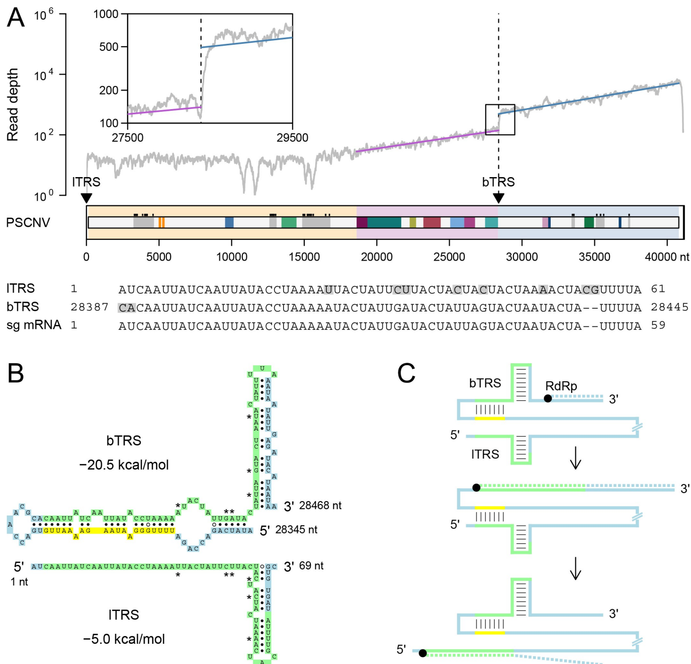
Fig 10. Genome transcription. (A) Mean depth of RNA-seq coverage along the PSCNV genome (approximated by exponential regression in ORF1b-like and 3'ORFs-like regions) calculated based on five datasets used to assemble the transcriptomes in which PSCNV was found [67]. Indicated on the genome map (colored as in Fig 2) are the positions of oligonucleotide repeats (leader and body TRSs) in the genome, and below is their alignment with a sg mRNA 5'-terminus identified by 5'-RACE (nucleotide mismatches between sg mRNA and TRSs are shown with grey backgrounds). (B) Predicted secondary structure of TRSs. TRSs are highlighted in green, region upstream of bTRS, interacting with its 5'-terminus—in yellow, asterisks indicate mismatching nucleotides of TRSs. (C) Model of discontinuous RNA synthesis mediated by TRSs and their secondary structure. The genome is represented by a solid line, and the nascent minus strand by a dashed line. Color code matches that of panel B.
