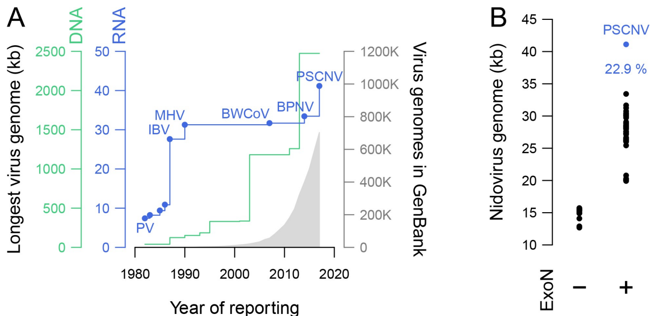
Fig 1. Genome sizes of nidoviruses. (A) Timeline of discovery of largest RNA and DNA virus genomes versus accumulation of virus genome sequences in GenBank (1982–2017). PV, poliovirus; and nidoviruses: IBV, avian infectious bronchitis virus, MHV, mouse hepatitis virus, BWCoV, beluga whale coronavirus SW1, BPNV, ball python nidovirus and PSCNV, planarian secretory cell nidovirus. (B) Comparison of genome sizes between nidoviruses that do not encode an ExoN domain, and those that do. Percentage indicates the difference between sizes of PSCNV and the next-largest entity.
