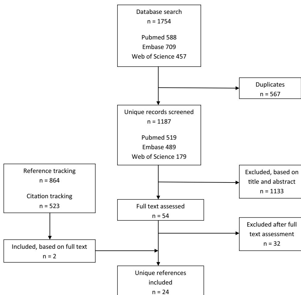
Fig. 2 Flowchart—prognosis
