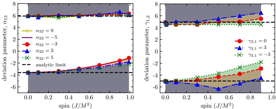
FIG. 1. Bound on the deviation parameters ( Left ) \alpha_{13} of the JP metric and ( Right ) \gamma_{1,2} for the MGBK metric, as a function of spin ( J/M^2 ) and for different values of the other metric parameters, placed by the 2017 EHT observations of M87. The shaded areas show the excluded regions of the parameter space. The dashed line shows the analytic result obtained for zero spin. The EHT measurements place constraints predominantly on \alpha_{13} (for JP) and \gamma_{1,2} (for MGBK), which control the 2PN expansion of the corresponding metrics (see Table I).
