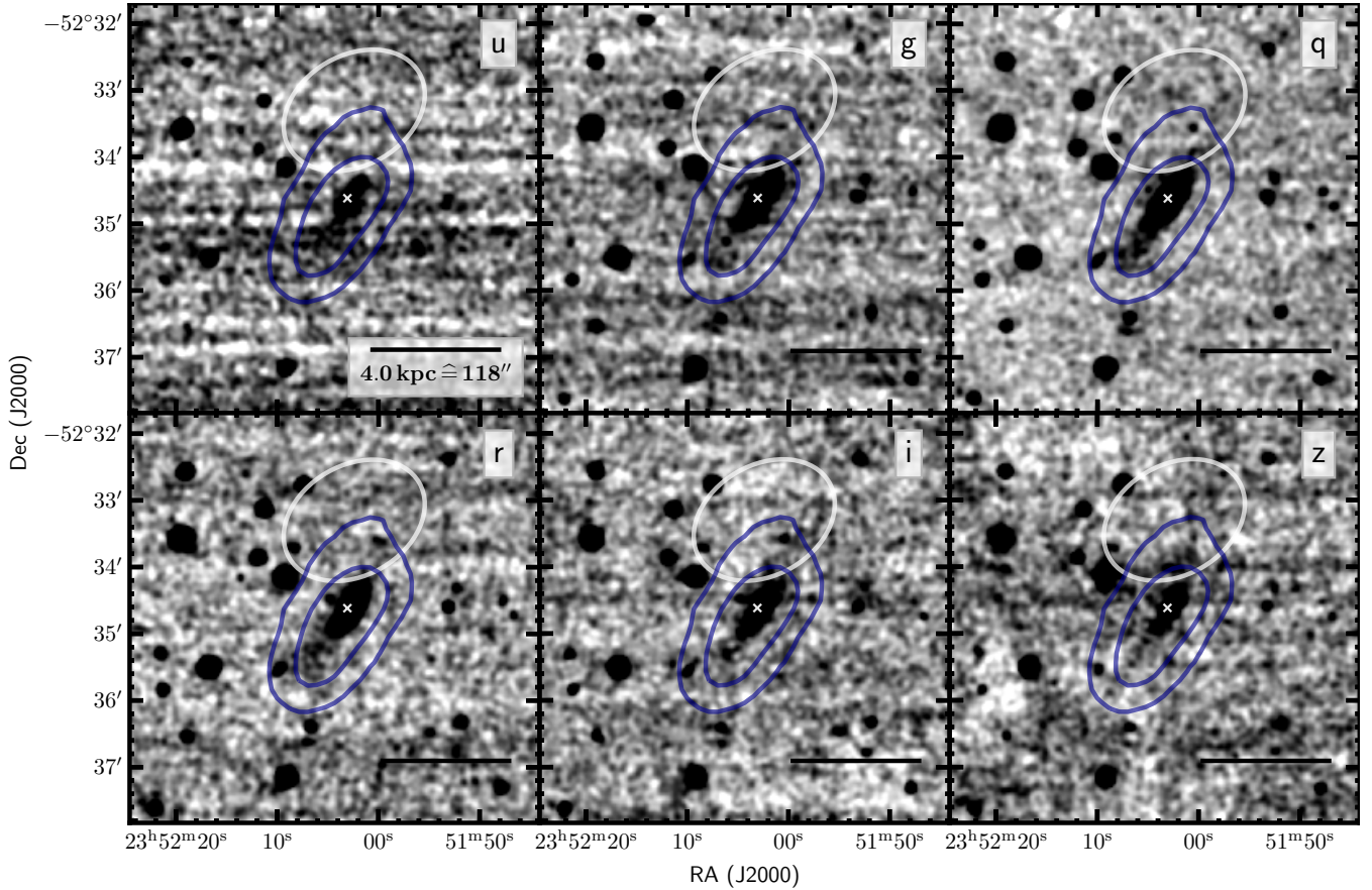
Figure 4. MeerLICHT observations of ESO 149-G003, convolved with a 2D-Gaussian of FWHM = 6'' in each direction (RA and Dec). Contours denote the 1, 4 M_{\odot} \text{pc}^{-2} -levels of the observed total-intensity map shown in the left panel of Figs. 3 and A3. The white ellipse to the top highlights kinematically anomalous gas. The white cross represents the kinematical centre of the kinematical model. The full-resolution maps can be found in Fig. A6 in the appendix.
