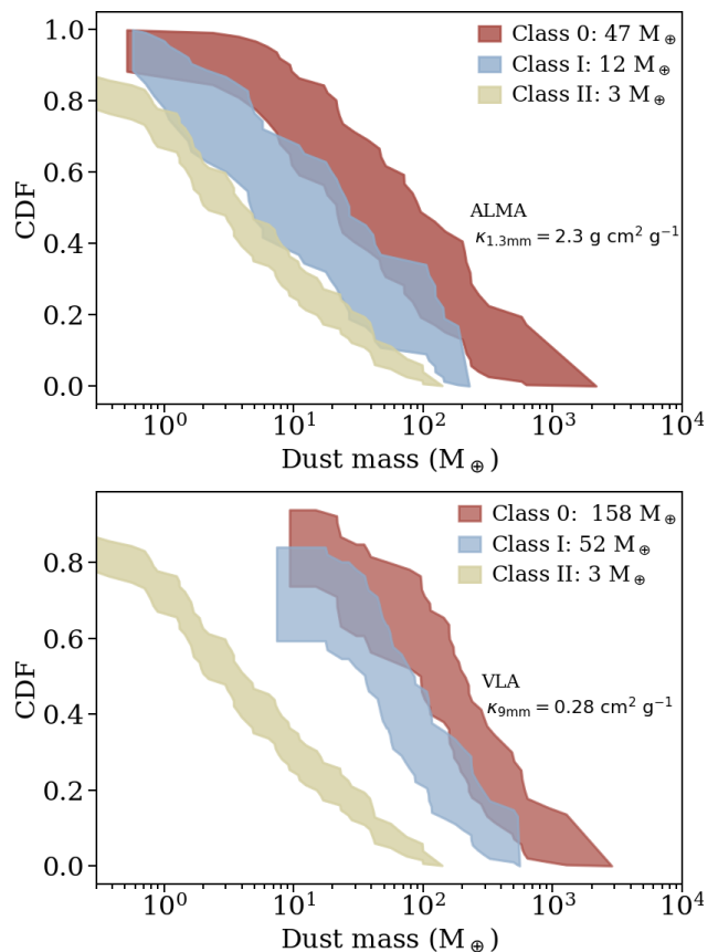
Fig. 2: Cumulative distribution plots of the dust disk masses. Top : Masses of the Perseus Class 0 and I disks measured with ALMA at 1 mm compared with the Lupus Class II disks measured with ALMA (Ansdell et al. 2016). The opacity value of \kappa_{1.3\text{mm}} = 2.3 \text{ cm}^2 \text{ g}^{-1} is used to calculate the masses. The ALMA sample consist of 77 sources (38 Class 0 and 39 Class I) and the Lupus sample consist of 69 sources. Bottom : Masses of the Perseus Class 0 and I disks measured with VLA at 9 mm (red and blue, respectively), compared with the Lupus Class II disks measured with ALMA (Ansdell et al. 2016). The opacity value of \kappa_{9\text{mm}} = 0.28 \text{ cm}^2 \text{ g}^{-1} is used to calculate the VLA masses. The VLA sample consist of 100 sources (49 Class 0 and 51 Class I). Medians are indicated in the labels.
