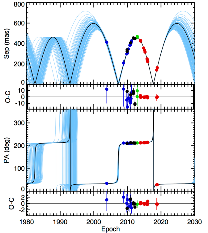
Figure 8. Orbit tracks for the orbit fit to both the imaging and astrometric datasets (Case 3). While the uncertainty in eccentricity remains, with zero eccentricity orbits no longer allowed, longer orbital periods are preferred.
