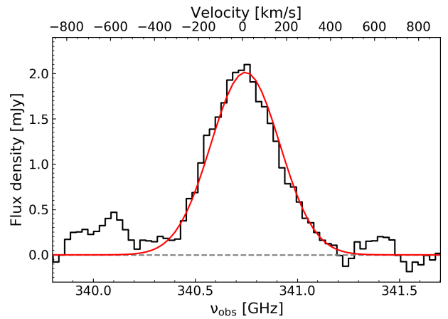
Figure 2. Emission line flux at the position of Gal-A (black histogram) as a function of the observed frequency. The solid red curve represents the gaussian fit on the line. The dashed grey line marks the zero-flux level. Also shown is the velocity offset on the top axis.
