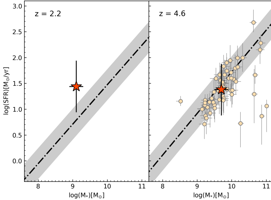
Figure 6. Star-forming MS relations (dot-dashed lines; Speagle et al. 2014 ) at redshift 2.2 (left panel) and 4.6 (right panel). The grey bands indicate the scatter from the MS ( \pm 0.3 dex width). The orange stars represent the positions of our source in the diagram, given by the estimated stellar mass from the SEDfitting and the SFR from the FIR luminosity of Gal-A. For the case at z = 4.6 , we also show the positions of the ALPINE galaxies at 4.4 \leq z \leq 4.6 (small circles).
