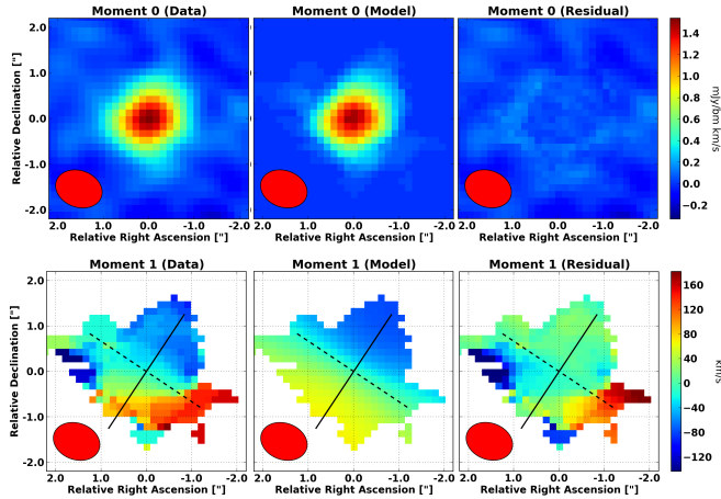
Figure 9. The best-fit 3D modeling results in the moment 0 (top) and moment 1 (bottom) maps for VC5110377875 with 3D Barolo (Di Teodoro & Fraternali 2015). The observed, the best-fit model, and the residual maps are presented from left to right. The solid and dashed lines are drawn along with the kinematic major and its perpendicular axes. The systematic 3D modeling results for the entire ALPINE sample are presented in Jones et al. in (prep.).
