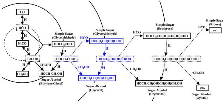
Figure 5. Reaction scheme leading to complex sugars in ices at low temperatures (10-15 K), without the need for UV radiation or cosmic rays. Figure from Fedoseev et al. (2017).
