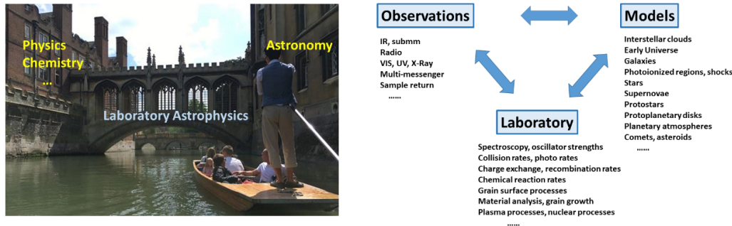
Figure 1. Left: The Bridge of Sighs in Cambridge (UK), symbolizing laboratory astrophysics as a bridge between astronomy and physics, chemistry and other sciences. Credit: Tripadvisor.co.uk. Right: the triangle of observations, models and laboratory astrophysics, with the latter underpinning both.
