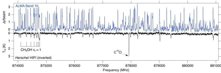
Figure 3. ALMA Band 10 spectrum of the high-mass star-forming region NGC 6334I, compared with the spectrum over the same frequency range obtained with Herschel . Note the huge number of lines detected with ALMA due to its much smaller beam. Around 20-70% of ALMA lines are still unidentified, stressing the need for more laboratory spectroscopy. Figure based on McGuire et al. (2018a).
