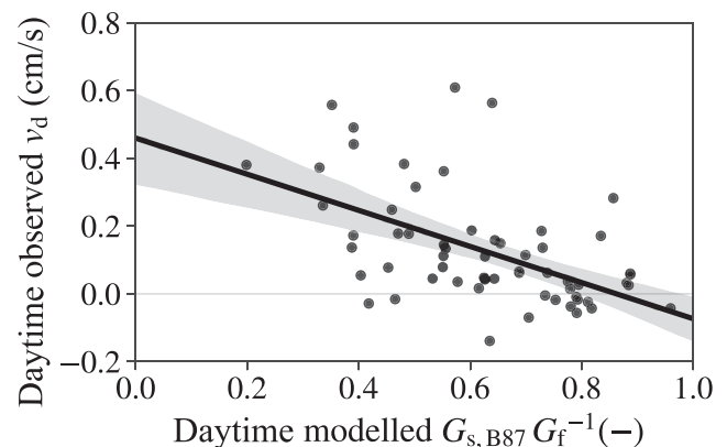
FIGURE 3 Linear regression of observed daily mean daytime \text{NH}_3 dry deposition velocities against daytime ratio of \text{CO}_2 flux-derived stomatal conductance to total modelled foliar conductance. One outlier ( v_d > 1.5 cm/s on 25 February 2014) was removed from the regression data set. The shaded area envelopes a 95% confidence interval of the regression based on 10,000 bootstrap samples
