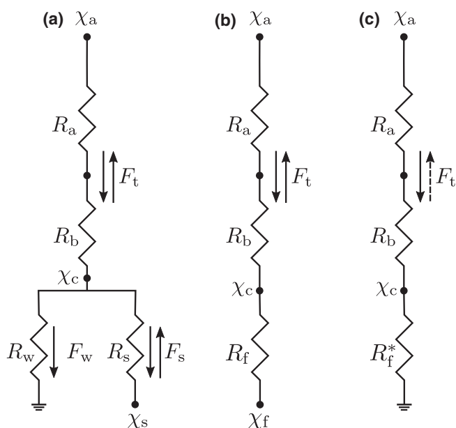
FIGURE 1 (a) Common structure of a canopy compensation point model with a unidirectional non-stomatal and a bidirectional stomatal \text{NH}_3 exchange pathway. (b) Serial bidirectional simplification with foliar resistance and foliar compensation point. (c) Serial unidirectional simplification with effective foliar resistance
