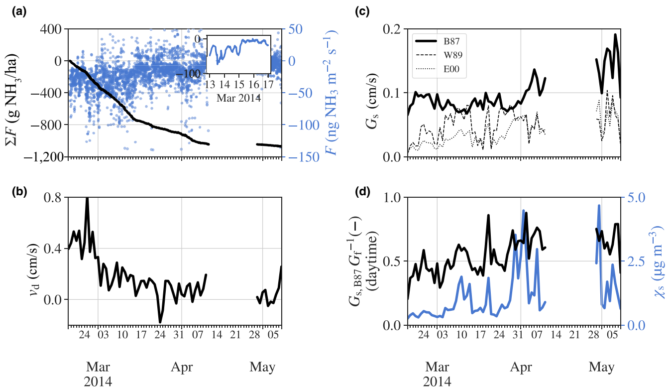
FIGURE 2 Results from the 'Bourtanger Moor' case study. (a) Half-hourly \text{NH}_3 mass flux density (blue dots) and gap-filled cumulative \text{NH}_3 flux (black line) obtained with eddy covariance measurements. Small inset shows sudden decline in 6 hr moving average flux densities around 15 March. Negative fluxes indicate deposition. (b) Observed daily average \text{NH}_3 dry deposition velocity. (c) Modelled daily average stomatal conductance obtained from two empirical models (W89: Wesely, 1989; E00: Emberson et al., 2000) and from eddy covariance fluxes of \text{CO}_2 using the Ball–Woodrow–Berry model (B87: Ball et al., 1987) (d) Daily average contribution of stomatal conductance to total foliar conductance (black line) and stomatal compensation point (blue line) during daytime using the Ball–Woodrow–Berry model
