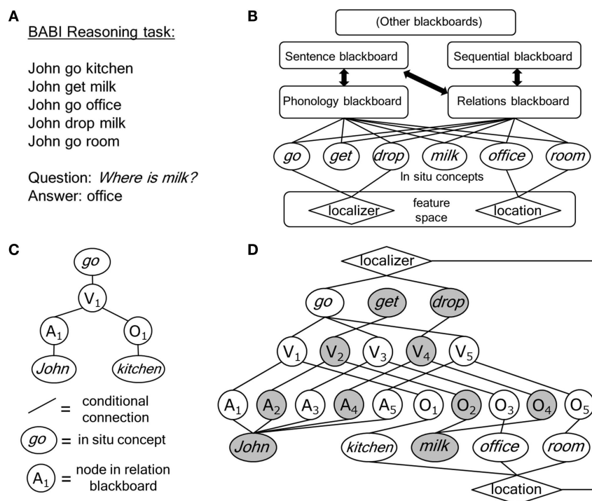
FIGURE 1 | (A) An example of a BABI reasoning task [after Bordes et al. (2015)]. (B) Architecture for in situ concept computing, consisting of a set of identified and not yet identified (“other”) blackboards (ovals represent in situ concepts). (C) Representation of John go kitchen in the in situ concept architecture of (B) (circles represent nodes in the reasoning blackboard; A, actor; V, verb; O, object). (D) Activation (gray nodes and ovals) in the in situ concept architecture of (B) initiated by the question Where is milk?
