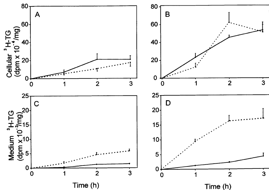
Figure 4. Time-dependent accumulation of [ ^3\text{H} ]TG in apo E-deficient and control hepatocytes and secretion of [ ^3\text{H} ]TG-VLDL by these cells. After their isolation, apo E-deficient ( solid line ) and control (C57BL/6J) hepatocytes ( dotted line ) were cultured overnight in FCS and hormone-containing media. Cells were washed thoroughly and incubated for an additional 4 h in FCS and hormone-free medium. Subsequently, cells were incubated with medium containing BSA in the absence (A and C) or presence (B and D) of 0.75 mM oleate. [ ^3\text{H} ]Glycerol was added to label newly synthesized TG, as outlined in Methods. At the indicated time points, cells and media were harvested, and the accumulation of cellular [ ^3\text{H} ]TG (A and B) and secretion of [ ^3\text{H} ]TG-VLDL (C and D) were determined as described in Methods. A representative experiment is shown in which cells isolated from a single apo E-deficient mouse and a control mouse were studied simultaneously. Values are expressed as the mean \pm SD of triplicate determinations at each time point.
