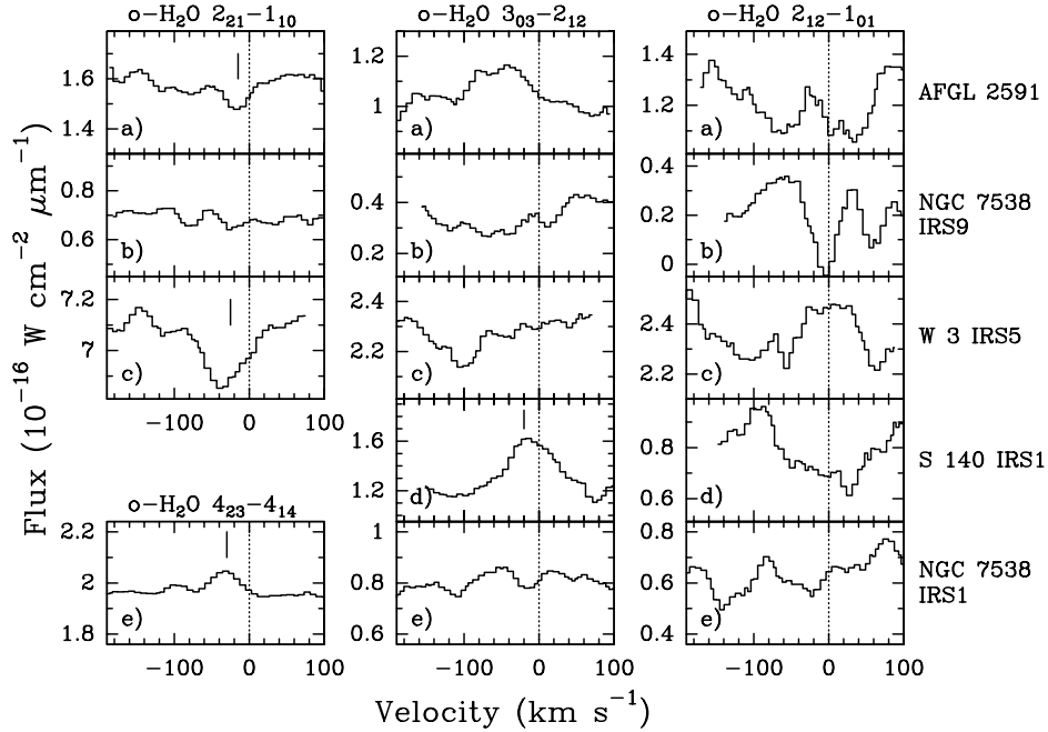
Fig. 1. Overview of the ISO-LWS data for a selection of the ortho-H 2 O 2_{21}-1_{10} , 4_{23}-4_{14} , 3_{03}-2_{12} , and 2_{12}-1_{01} lines at 108.1 \mu m, 132.4 \mu m, 174.6 \mu m, and 179.5 \mu m respectively, in a) AFGL 2591, b) NGC 7538 IRS9, c) W 3 IRS5, d) S 140 IRS1, and e) NGC 7538 IRS1. The vertical markers indicate the (tentative) detections. All lines have been corrected for the V_{\text{LSR}} of the source and the resolution of the spectra is \Delta V \sim 30 \text{ km s}^{-1} . The vertical dotted lines indicate the positions of the H 2 O lines if they are at the V_{\text{LSR}} of the source. The deviations of the (tentative) detections from the dotted lines are about the spectral resolution. The ortho-H 2 O 2_{21}-1_{10} line has not been observed toward S 140 IRS1. Note that the flux scale in the panel of the 3_{03}-2_{12} line in S 140 IRS1 covers twice as large a range as in all other panels.
