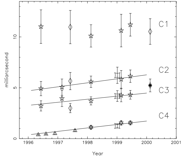
Fig. 12. Apparent proper motion of the jet components: 1.6 GHz (diamond), 5 GHz (star), 15 GHz (square), 22 GHz (triangle, Jorstad et al. 2001).
