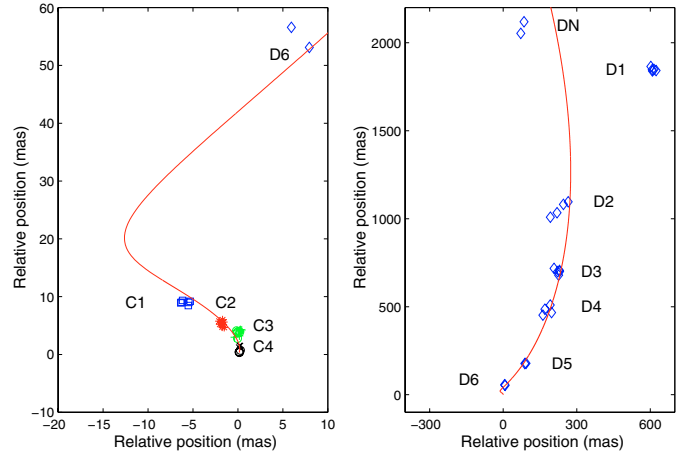
Fig. 17. The positions of jet components and the projective path of a helical jet in the image plane on the pc-(left) and the kpc-(right) scales.
