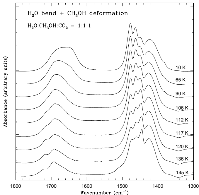
Fig. 13. Infrared absorption spectra of the H 2 O bending mode and the CH 3 OH deformation mode in a H 2 O:CH 3 OH:CO 2 = 1:1:1 mixture during warm-up. The deformation band of CH 3 OH consists of 4 peaks: three narrow peaks at \sim 1477 cm -1 , 1462 cm -1 and 1450 cm -1 and a broad shoulder at \sim 1420 cm -1 . For the 1450 cm -1 peak we find a redshift of \sim 5 cm -1 during warm-up, whereas the other bands are stable in position. The slope of the three narrow peaks is inverted during warm-up. The H 2 O bend appears broad at 10 K and decreases in width during warm-up. At 112 K a second band develops at the blue wing at 1720 cm -1 (5.81 \mu m).
