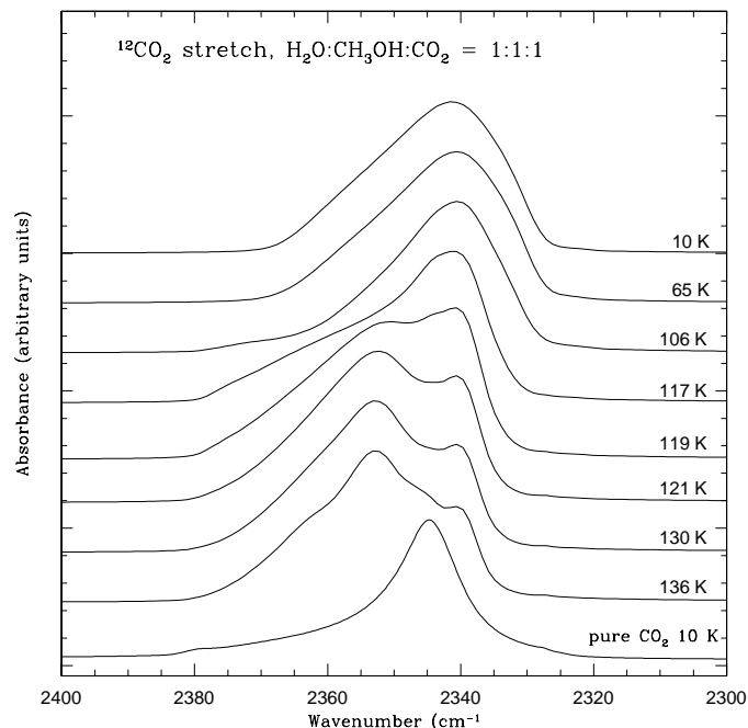
Fig. 7. Infrared absorption spectra of the 12 CO 2 stretch in a H 2 O:CH 3 OH:CO 2 = 1:1:1 mixture during warm-up up to 136 K. At 10 K we observe a single peak centered at \sim 2341 cm -1 which is characterized by a large band width of 24 cm -1 . At 117 K a second peak starts to arise as a blue wing probably due to aggregate formation. With increasing temperature the 2341 cm -1 peak decreases in strength. As comparison we show pure CO 2 centered at 2345 cm -1 with a band width of 12 cm -1 .
