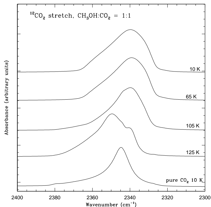
Fig. 3. Infrared absorption spectra of the ^{12}\text{CO}_2 stretch in a \text{CO}_2:\text{CH}_3\text{OH} = 1:1 mixture during warm-up to 125 K. At 10 K we observe a single peak centered at \sim 2340\text{ cm}^{-1} which is characterized by a large band width of 26\text{ cm}^{-1} . During warm-up a second peak starts to arise and becomes dominant at 125 K. As comparison we show pure \text{CO}_2 centered at 2345\text{ cm}^{-1} with a band width of 12\text{ cm}^{-1} .
