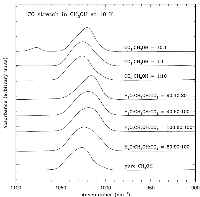
Fig. 14. Infrared absorption spectra of the CO stretch in CH 3 OH at 10 K. The band width varies between 26.4 cm -1 and 35.5 cm -1 and the position varies between 1026 cm -1 and 1016 cm -1 .
