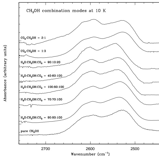
Fig. 15. Infrared absorption spectra of the combination modes of solid CH 3 OH in various matrices containing also CO 2 and H 2 O admixtures. The profile shape does not change significantly for the selected mixtures. A strong blueshift of \sim 20 cm -1 is observed in the mixture with high H 2 O abundance.
