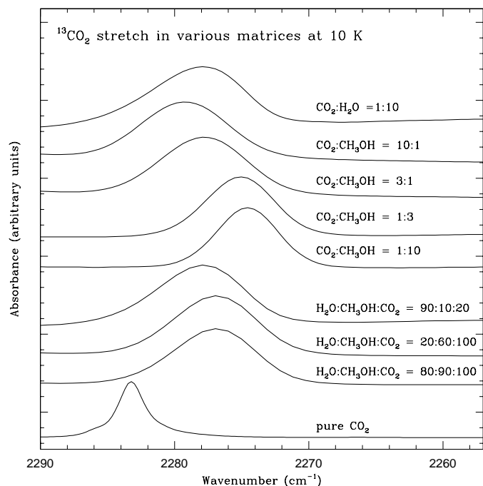
Fig. 11. Infrared absorption spectra of the 13 CO 2 stretch in various matrices at 10 K. The addition of other molecules to CO 2 ice results in an increased band width varying between 5.8 and 9.8 cm -1 . The mixtures containing CH 3 OH in abundance display a redshift of \sim 8 cm -1 compared to pure 13 CO 2 . Pure 13 CO 2 is known to have a very narrow band width of 2.4 cm -1 .
