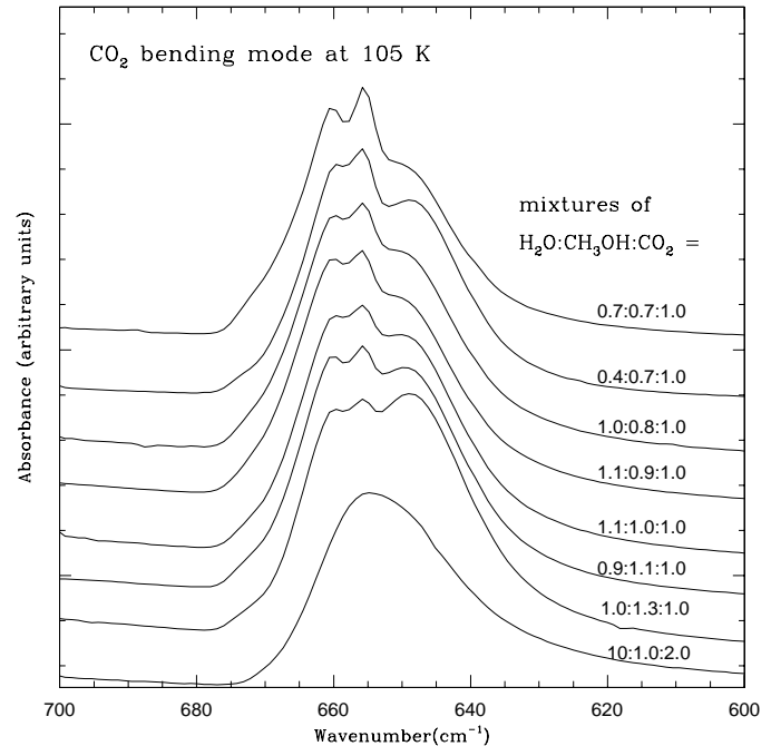
Fig. 9. Infrared absorption spectra of the CO 2 bending mode in annealed H 2 O:CH 3 OH:CO 2 mixtures. The profiles consist of two peaks at ~ 660 cm -1 (15.15 μm) and 656 cm -1 (15.24 μm) and a shoulder at ~ 648 cm -1 (15.4 micron). For increasing amounts of CH 3 OH relative to H 2 O and CO 2 , this shoulder grows and becomes equal or larger than the other two peaks. This implies that the absorption at 648 cm -1 is due to complexes between CO 2 and CH 3 OH (Ehrenfreund et al. 1998, Dartois et al. 1999b). A smaller abundance of H 2 O enhances the shoulder at 15.4 μm and leads to an increased band width.
