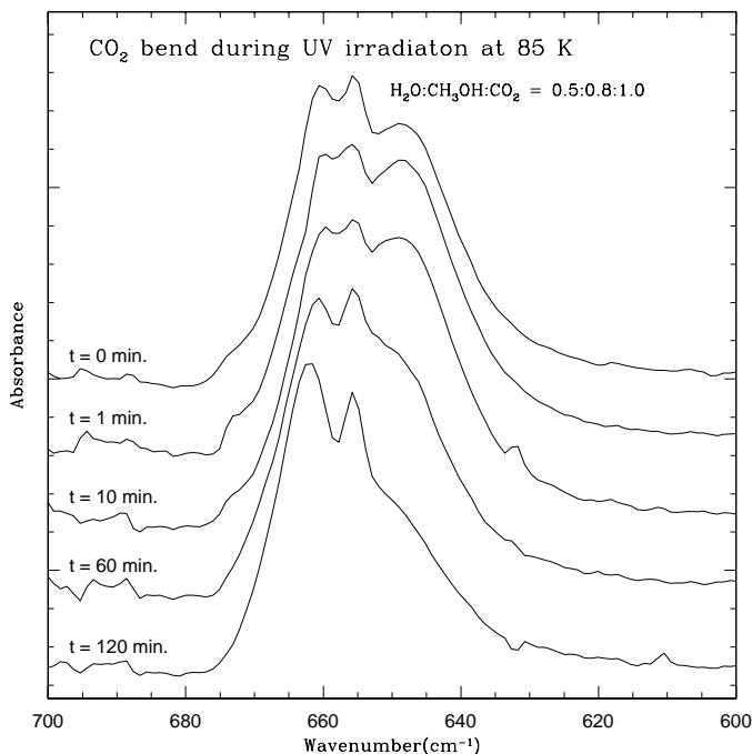
Fig. 18. Infrared absorption spectra of the CO 2 bending mode of an annealed H 2 O:CH 3 OH:CO 2 = 0.5:0.8:1.0 ice mixture displaying the triple peak. After two hours of UV irradiation 61% of the CH 3 OH and 33% of the CO 2 is destroyed. The shoulder at 648 cm -1 completely vanishes and the peak splitting increases.
