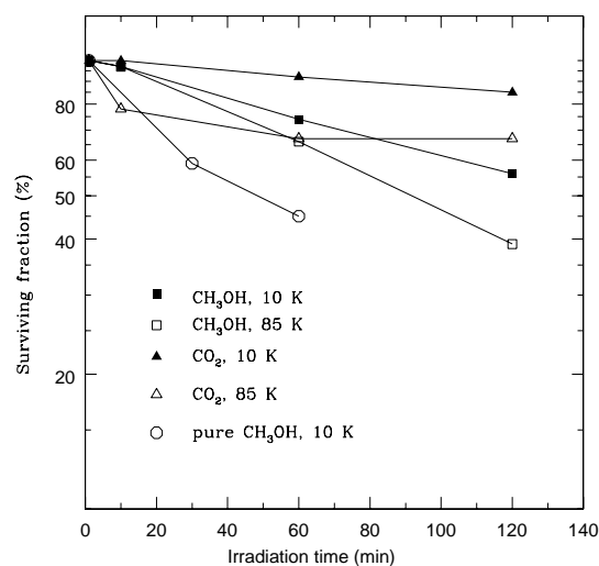
Fig. 16. Destruction of CH 3 OH and CO 2 during irradiation of a H 2 O:CH 3 OH:CO 2 = 0.5:0.8:1.0 mixture at 10 K and after warm-up to 85 K. Also displayed is the destruction of pure CH 3 OH.
