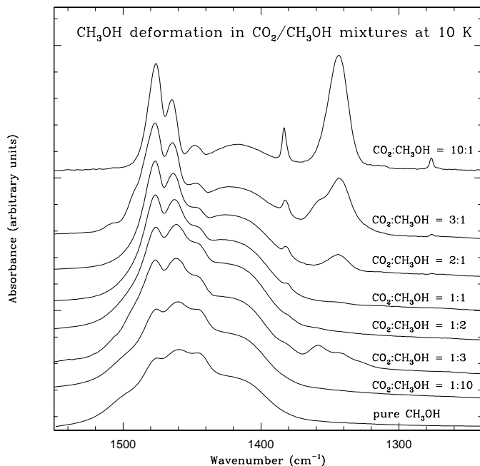
Fig. 6. Infrared absorption spectra of the CH 3 OH deformation in CO 2 /CH 3 OH mixtures at 10 K. The deformation mode consists of three narrow peaks at \sim 1475 cm -1 , 1465 cm -1 and 1447 cm -1 and a broad shoulder at \sim 1420 cm -1 . The structure of the triple-peak smoothens as the relative amount of CH 3 OH increases. The extra peaks at 1380 cm -1 , 1276 cm -1 and 1340 cm -1 are particularly strong in the mixture CO 2 :CH 3 OH = 10:1. They may be attributed to the infrared inactive CO 2 modes and isolated CH 3 OH, respectively.
