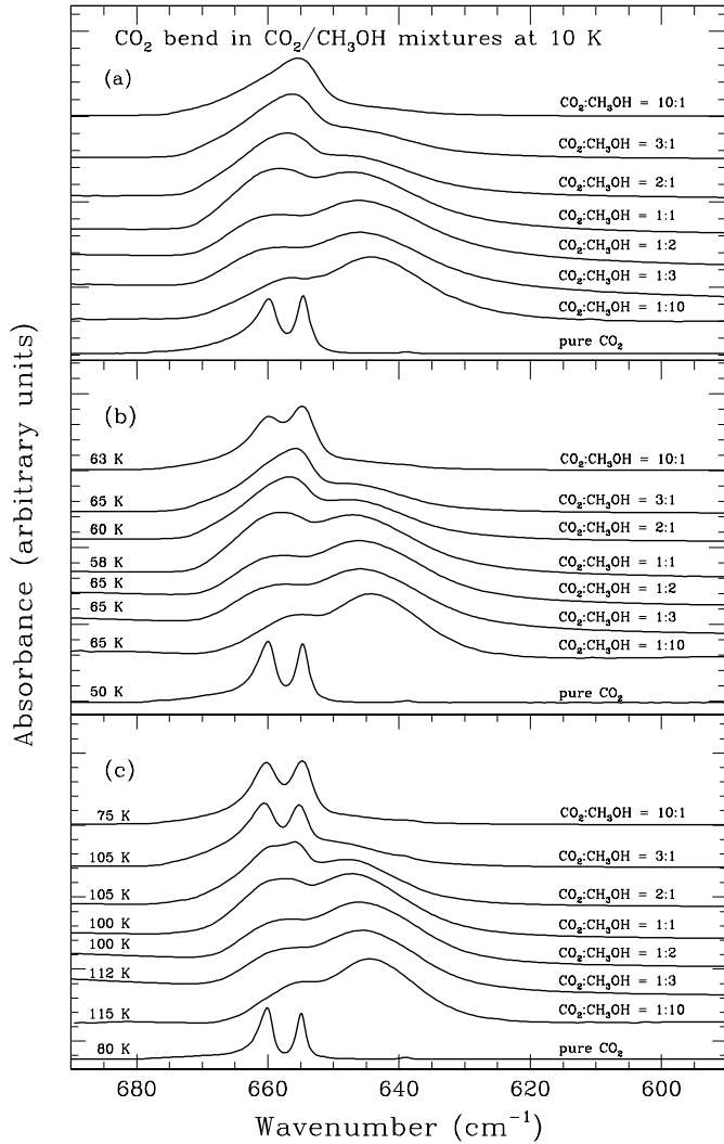
Fig. 4a–c. Infrared absorption spectra of the CO 2 bending mode in CO 2 /CH 3 OH mixtures at 10 K, ~60 K and ~100 K. In pure CO 2 the spectrum of the bending mode shows a double peak at 660 cm -1 and 655 cm -1 , respectively. a At 10 K the addition of 10% CH 3 OH shows a single peak at 655 cm -1 . When increasing the CH 3 OH content in the mixture, a second peak appears at ~ 648 cm -1 due to the formation of complexes. b At temperatures of ~60 K we observe the same behavior. The 10% CH 3 OH mixture shows a double peak indicating interaction between CO 2 molecules in the ice segregation process. c At temperatures of ~ 100 K we observe peak splitting for mixtures where CO 2 is abundant. CH 3 OH-dominated mixtures show similar profiles for all temperatures, due to their higher stability during thermal processing.
