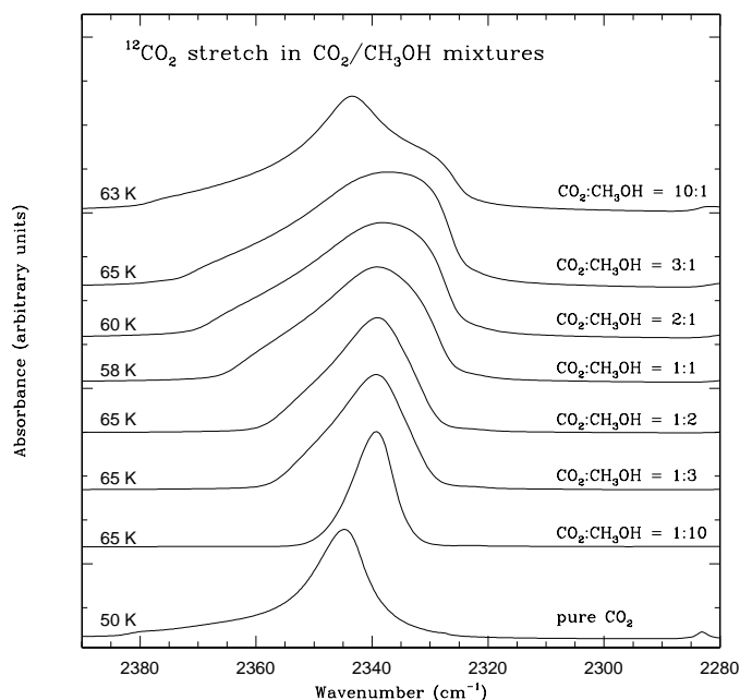
Fig. 2. Infrared absorption spectra of the ^{12}\text{CO}_2 stretch in \text{CO}_2/\text{CH}_3\text{OH} mixtures at \sim 60 K. All spectra show exactly the same profile as the 10 K measurements (compare Fig. 1). Only the \text{CO}_2:\text{CH}_3\text{OH} = 10:1 mixture shows a change in profile. This mixture is rather volatile and the ice matrix is rearranged at low temperatures.
