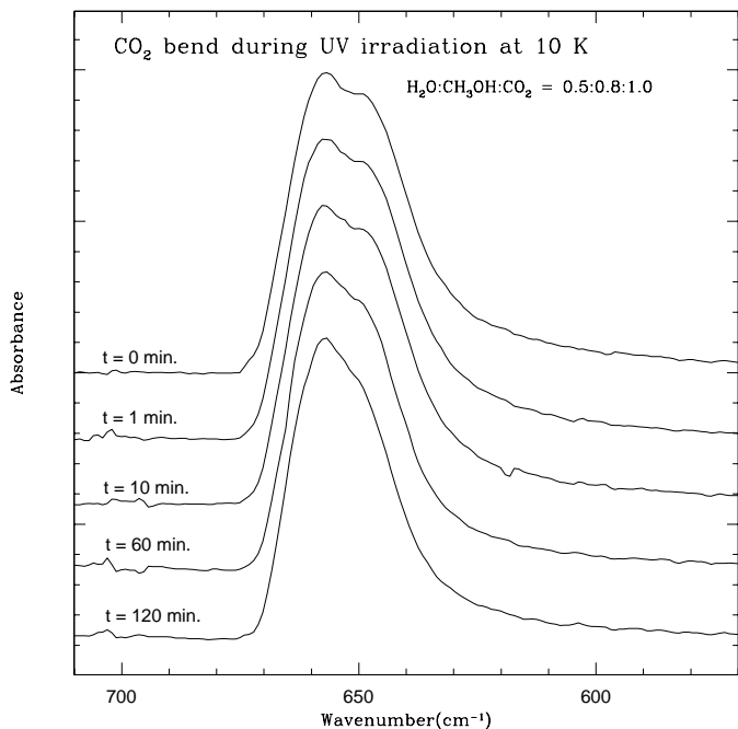
Fig. 17. Infrared absorption spectra of the CO 2 bending mode of a H 2 O:CH 3 OH:CO 2 = 0.5:0.8:1.0 ice mixture at 10 K during UV irradiation. After irradiation of two hours 44% of the CH 3 OH and 15% of the CO 2 is destroyed and we observe a noticeable decrease of the strength of the 648 cm -1 (15.4 μm) shoulder.
