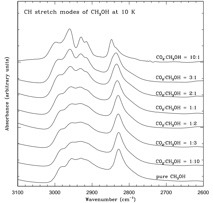
Fig. 5. Infrared absorption spectra of the CH stretching modes of solid CH 3 OH mixed with CO 2 . For the ν 9 stretch 4 peaks centered around 2960 cm -1 are observed. The narrow band at positions varying between 2847 cm -1 and 2827 cm -1 corresponds to the ν 3 stretch. The latter shifts toward lower frequencies as the CO 2 /CH 3 OH ratio decreases (see also Table 2). At the same time the multiplex structure of the ν 9 stretch at 2950 cm -1 (3.39 μm) becomes less pronounced.
