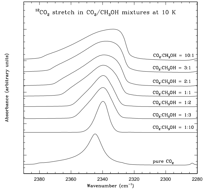
Fig. 1. Infrared absorption spectra of the 12 CO 2 stretch in CO 2 /CH 3 OH mixtures at 10 K. Addition of 10% CH 3 OH to CO 2 strongly broadens the band (FWHM of 37 cm -1 ) and results in a redshift of about 10 cm -1 . Increasing the amount of CH 3 OH shows a decrease in band widths of the CO 2 band. The band shifts at the same time toward higher frequencies. The difference in band position and width between CO 2 :CH 3 OH = 3:1 and 1:3 shows that the interactions between CH 3 OH and CO 2 are strongly related to their abundance ratio and that a higher abundance of CO 2 (see Table 1) leads to stronger perturbation (and aggregate formation) reflected in a large band width.
