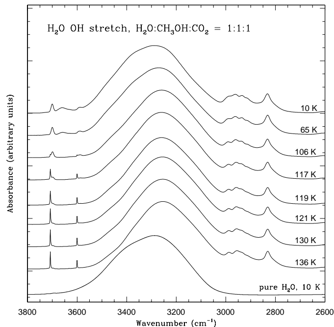
Fig. 12. Infrared absorption spectra of the OH stretching mode of H 2 O at 3290 cm -1 (3.0 \mu m) in an H 2 O:CH 3 OH:CO 2 = 1:1:1 mixture during warm-up. Annealing to 136 K results in a redshift of the OH stretch of H 2 O of 37 cm -1 . Isolated H 2 O and CH 3 OH bands around 3600 cm -1 disappear during warm-up. The overtones of CO 2 at 3700 cm -1 and 3600 cm -1 , blended at low temperature with isolated H 2 O and CH 3 OH bands, become sharper during warm-up and show a blueshift of \sim 10 cm -1 . At the red wing of the 3.0 \mu m band are the CH stretching modes of CH 3 OH (see Fig. 5).
