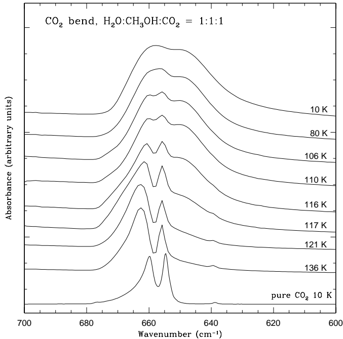
Fig. 8. Infrared absorption spectra of the CO 2 bending mode in an H 2 O:CH 3 OH:CO 2 = 1:1:1 mixture during annealing to 136 K. At 10 K the bending mode is characterized by a broad asymmetric profile with two shoulders at 658 cm -1 and 648 cm -1 . The peak at 658 cm -1 starts to split symmetrically at ~90 K. The magnitude of the low frequency shoulder decreases with increasing temperature and disappears spontaneously at 121 K.
