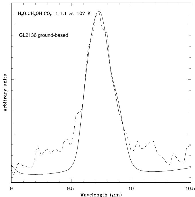
Fig. 19. The CO stretch of CH 3 OH at 9.7 \mu\text{m} ( 1026\text{ cm}^{-1} ) observed toward the YSO AFGL 2136 by Skinner et al. (1992) (dashed line) and a H 2 O-CH 3 OH-CO 2 mixture (solid line) in equal proportions, annealed to 107 K. The good fit indicates ice segregation and that CH 3 OH is not mixed with the bulk of H 2 O ice on grain mantles in the line-of-sight. The same mixture at 10 K does not fit these observations. The wings in the astronomical spectrum arise from smoothing the substantial noise at the continuum.
