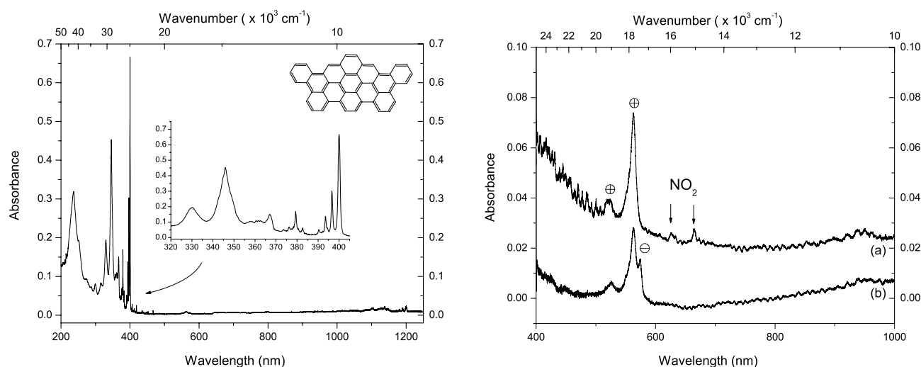
Fig. 8. Comparison of the spectral features associated with neutral (left panel) and VUV-irradiated (right panel) hexabenzoperopyrene (Hp) isolated in neon (Ne) and in Ne/NO 2 matrices. a) is the spectrum of the photolysis products in a neon/NO 2 matrix; b) is the spectrum of the photolysis products, including Hp + and Hp - , in a neon matrix. Band peak positions, intensities and FWHM are reported in Table 7.
