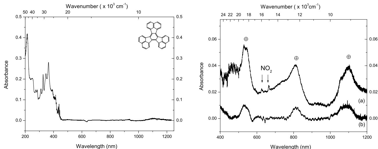
Fig. 5. Comparison of the spectral features associated with neutral (left panel) and VUV-irradiated (right panel) decacyclene (Dc) isolated in neon (Ne) and in Ne/ NO_2 matrices. a) is the spectrum of the photolysis products in a neon/ NO_2 matrix; b) is the spectrum of the photolysis products in a neon matrix. Band peak positions, intensities and FWHM are reported in Table 4.
