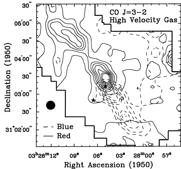
FIG. 3.—JCMT map of the CO J = 3 \rightarrow 2 high velocity outflow in the vicinity of NGC 1333/IRAS 4. The solid contours depict emission to the red of the systemic velocity, while the dotted contours outline the limits of the blue wing. Stars mark the positions of IRAS 4A and 4B as deduced from high-resolution millimeter-wave interferometric maps of the dust continuum emission (Mundy et al. 1995). Contour levels start at 2 \text{ K km s}^{-1} and are spaced by 2 \text{ K km s}^{-1} .
