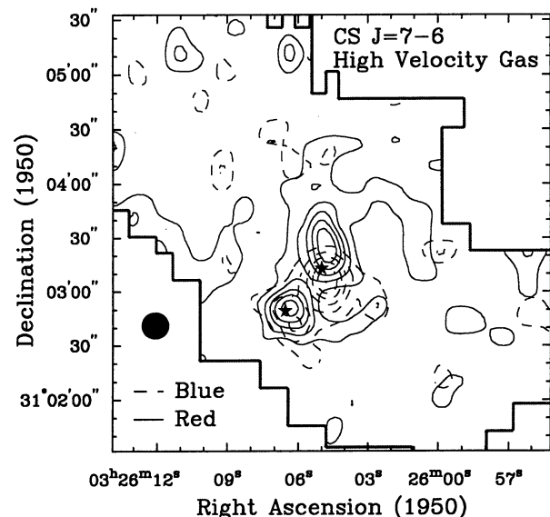
FIG. 4.—JCMT map of the CS J = 7 \rightarrow 6 outflow, in which the solid contours again depict the red wing, while the dotted contours outline the limits of the blue wing. The very high density structure of the inner structure of the CO 3 \rightarrow 2 map is clearly illustrated. Contour levels start at 0.3 \text{ K km s}^{-1} and are spaced by 0.3 \text{ K km s}^{-1} .
