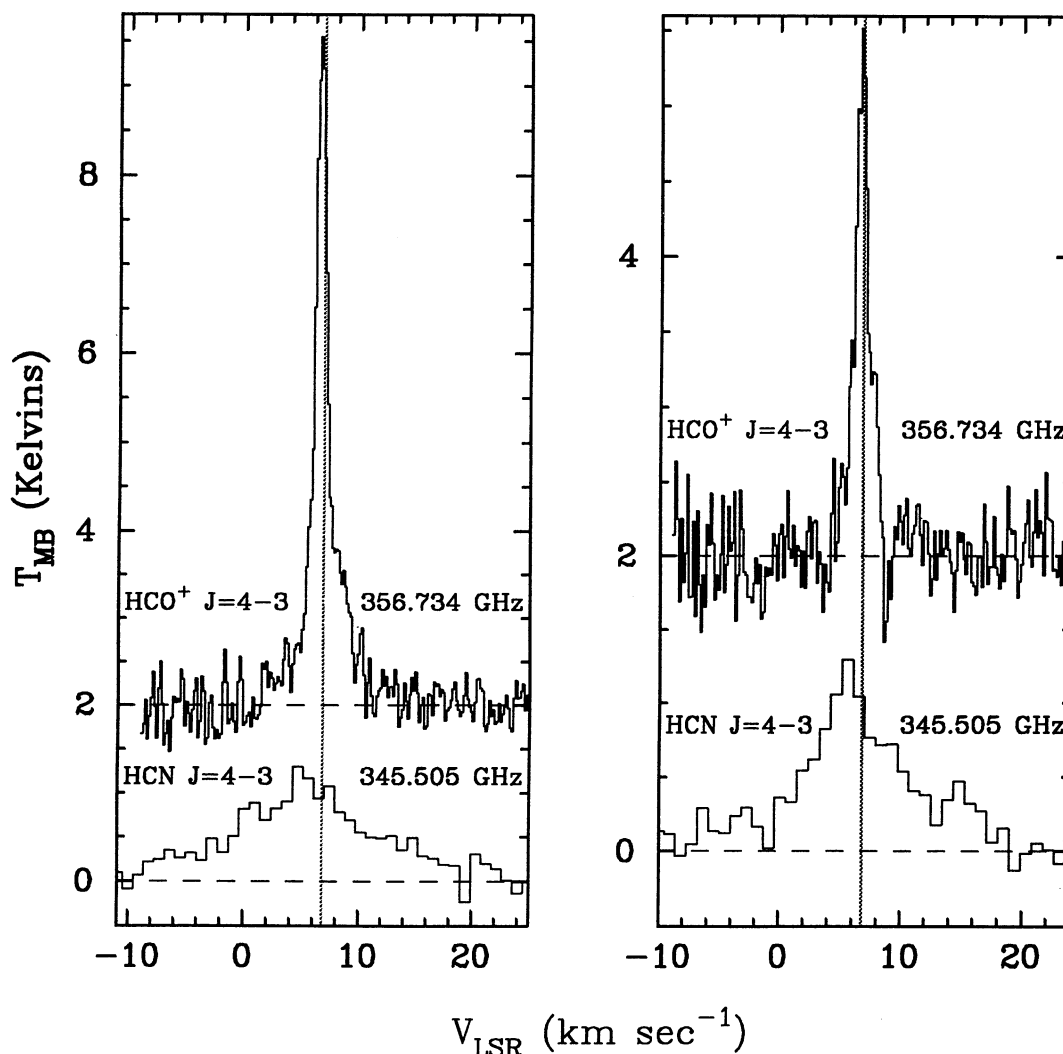
FIG. 8.—CSO spectra of the \text{HCO}^+ and \text{HCN } J=4 \rightarrow 3 transitions toward IRAS 4A (left) and 4B (right). Note that, despite the similar excitation requirements of these two transitions, \text{HCN} is largely devoid of the strong core emission present in the \text{HCO}^+ spectrum, while both species possess wing emission arising from the dense, outflowing gas.
